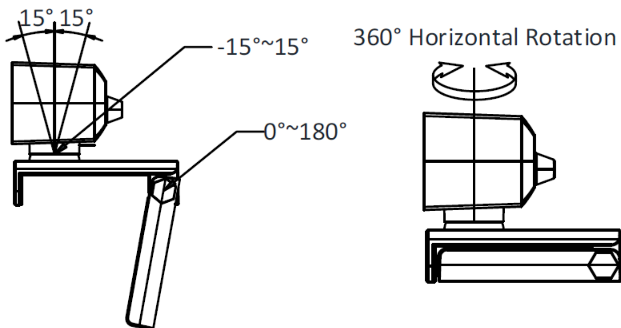
Figure 2-1 Angle Adjustment
