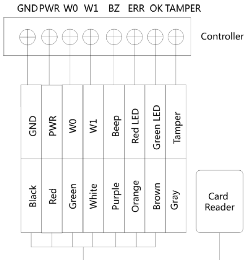
Figure 3-2 Wiring for Wiegand Communication Mode
