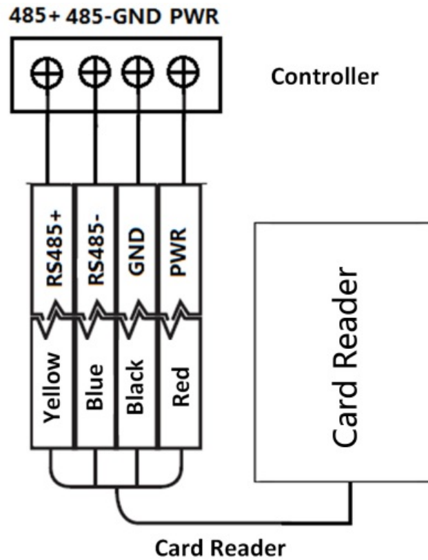
Figure 3-1 Wiring for RS-485 Communication Mode
