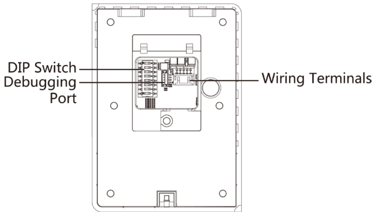
Figure 2-2 Rear View
