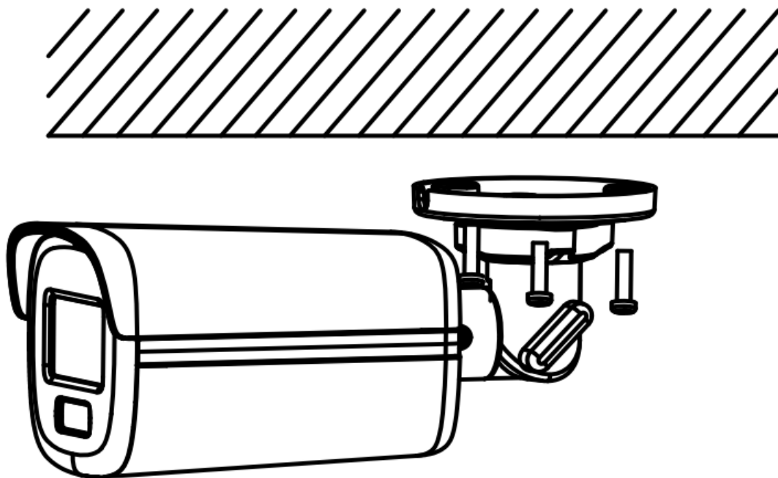
Figure 2-9 Secure the Camera to the Ceiling
