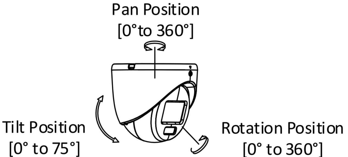
Figure 2-27 3-Axis Adjustment
