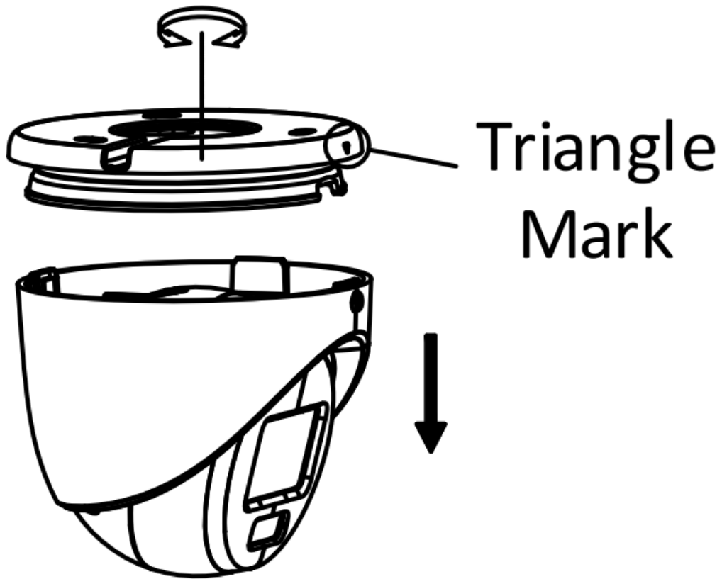
Figure 2-23 Disassemble the Camera
