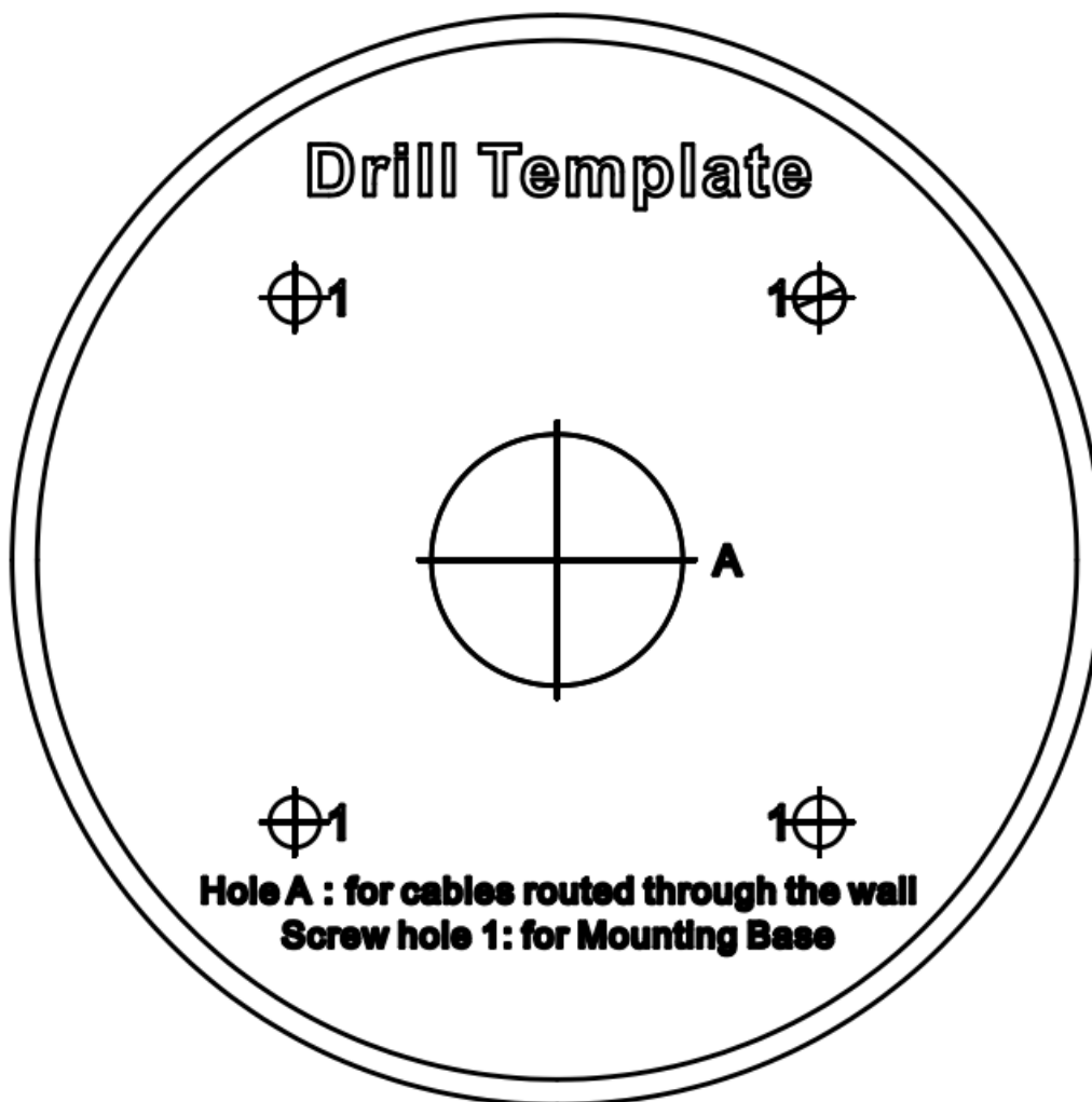
Figure 2-43 Drill Template
