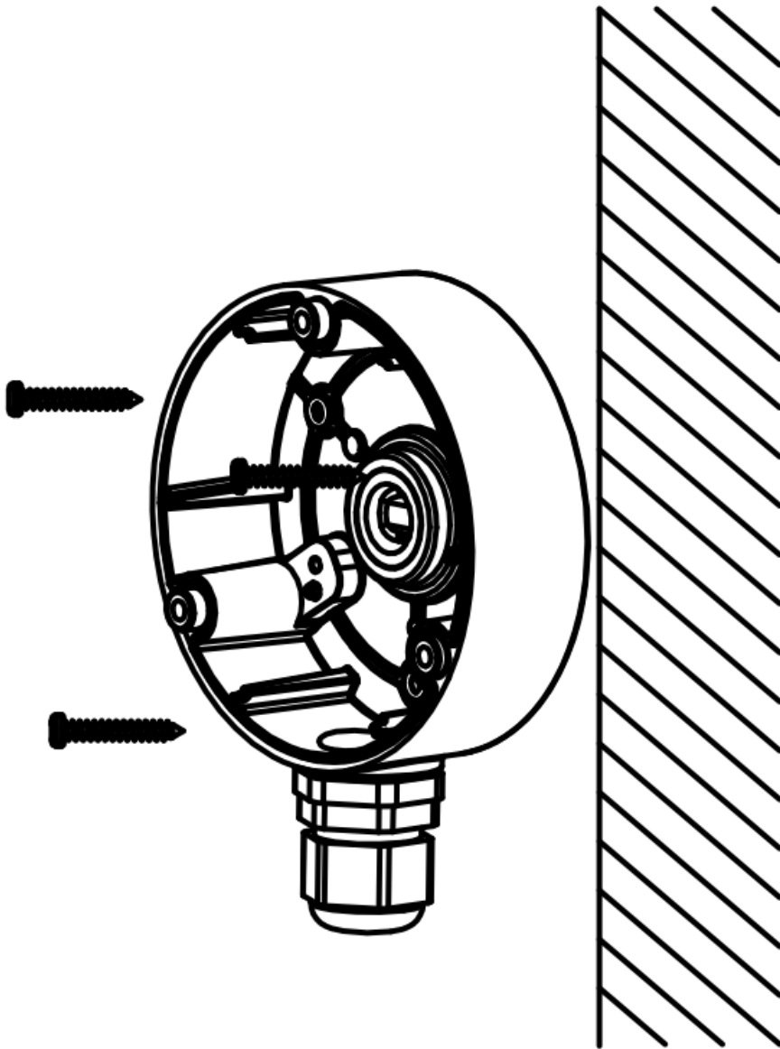
Figure 2-6 Secure the Junction Box on the Wall
