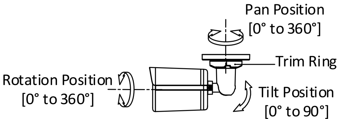
Figure 2-3 3-Axis Adjustment
