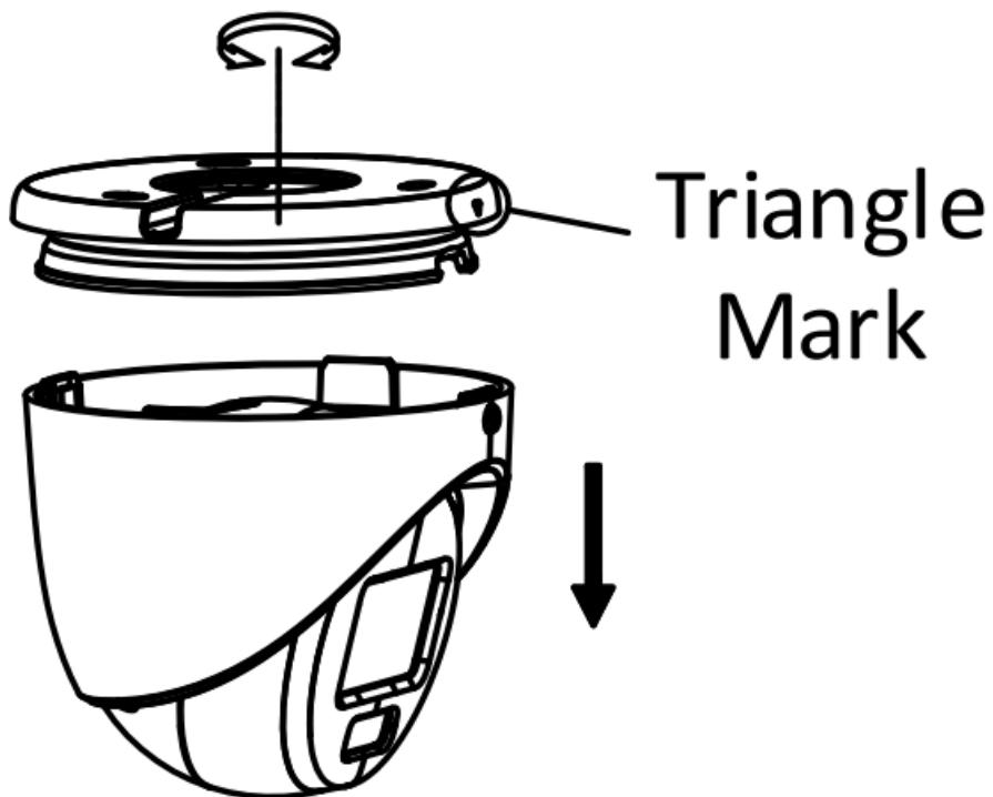
Figure 2-35 Disassemble the Camera
