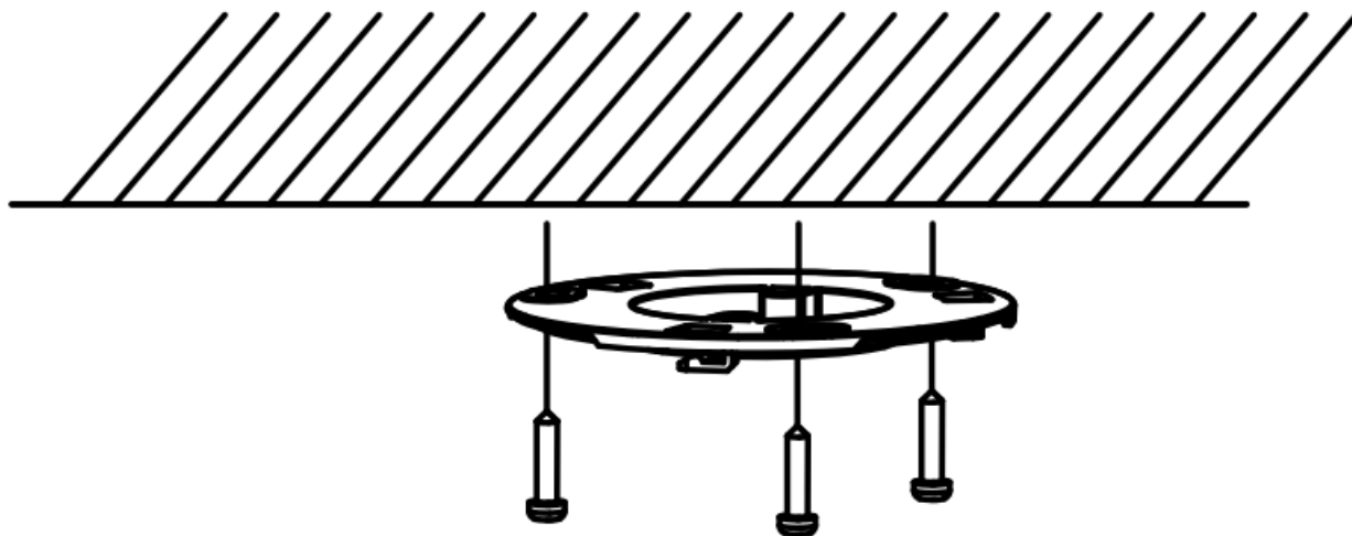
Figure 2-39 Attach the Gang Box to the Ceiling
