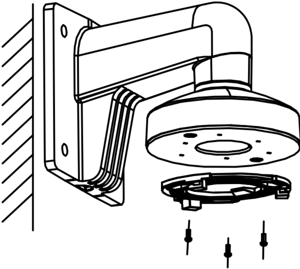
Figure 2-22 Finish the Installation
