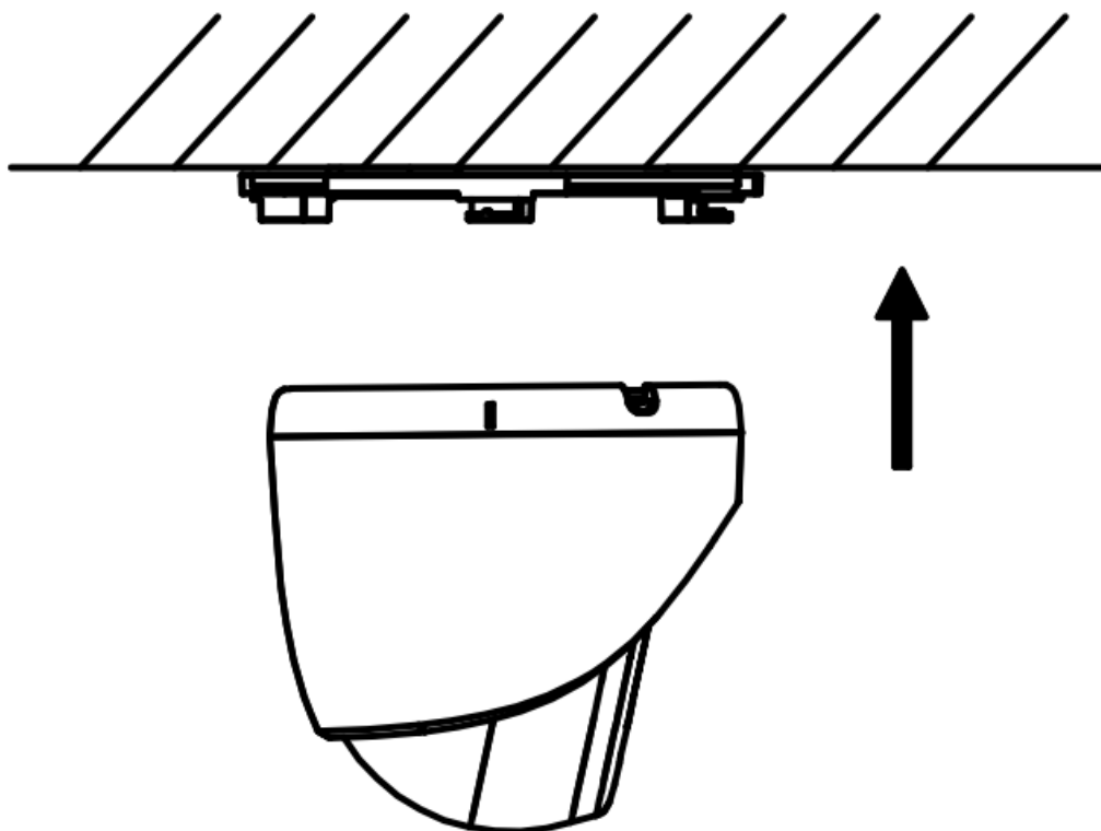
Figure 2-13 Fit the Camera onto the Gang Box
