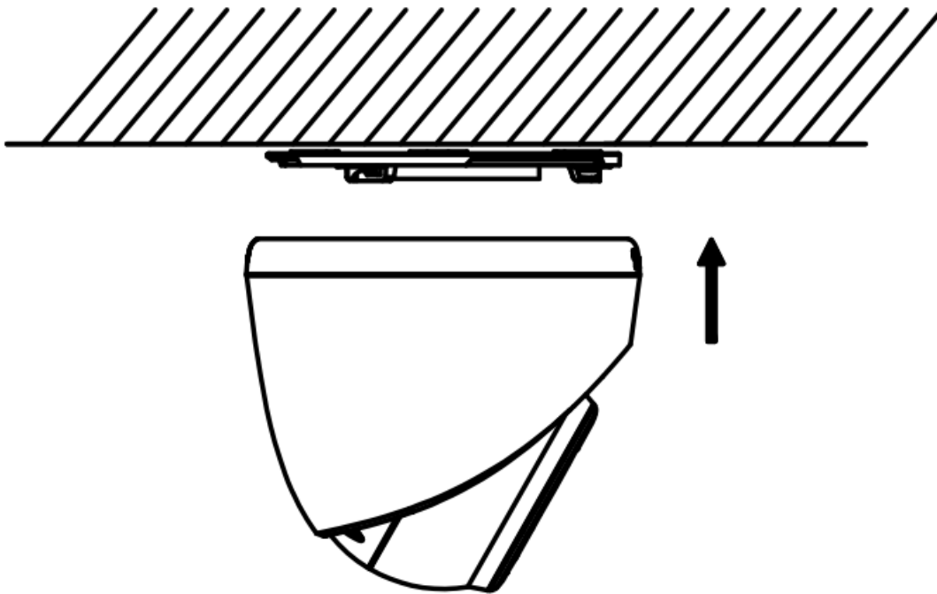
Figure 2-41 Snap the Camera into the Gang Box
