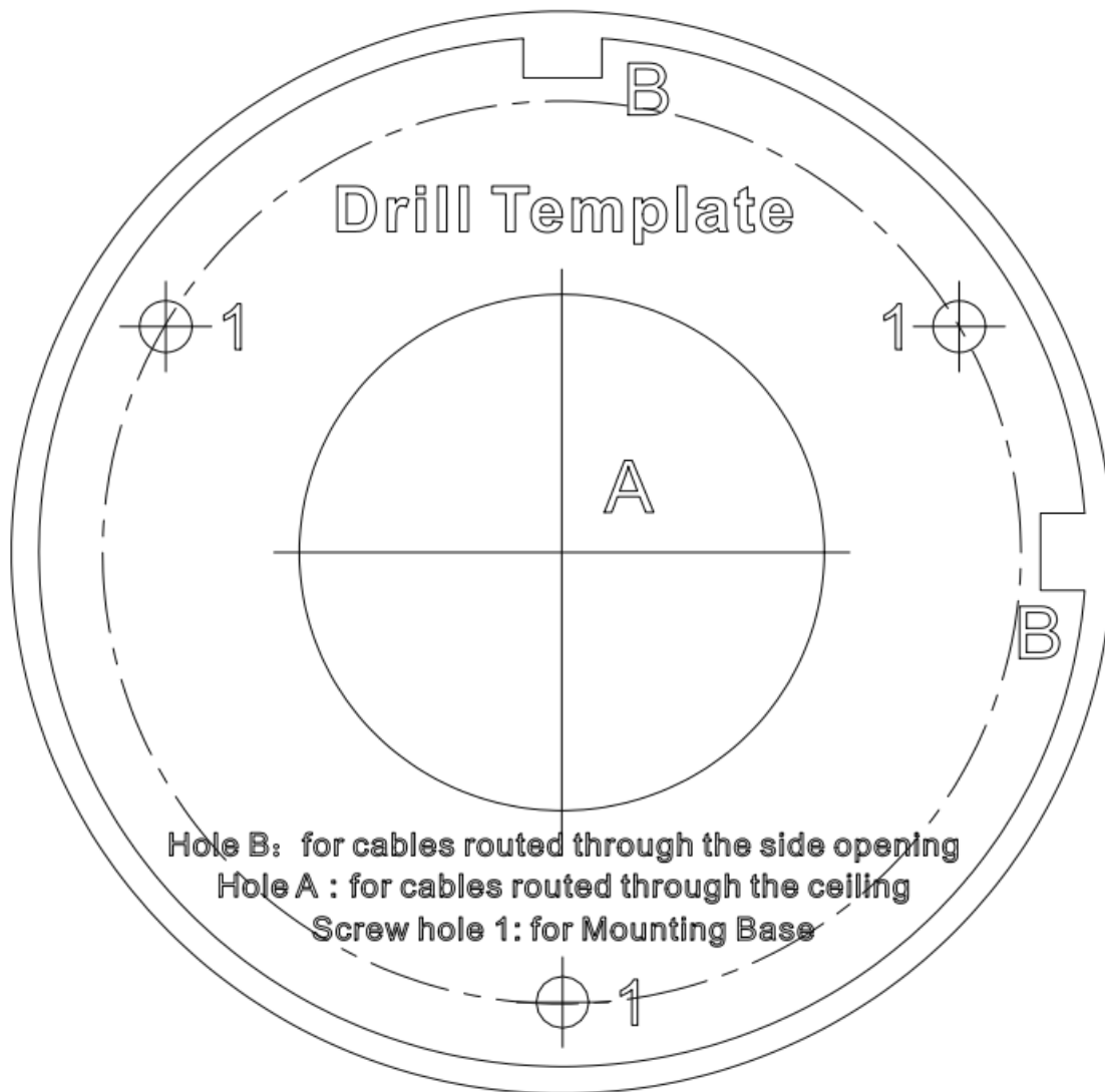
Figure 2-4 Drill Template for Junction Box
