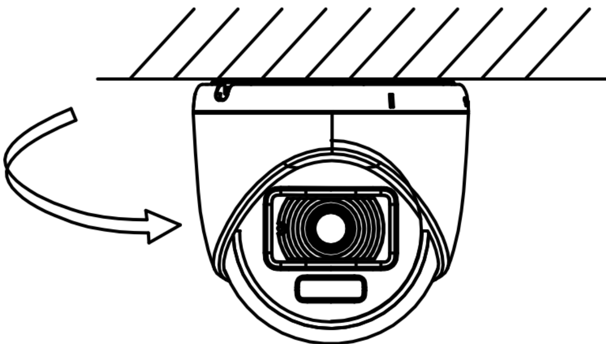
Figure 2-14 Snap the Camera into the Gang Box
