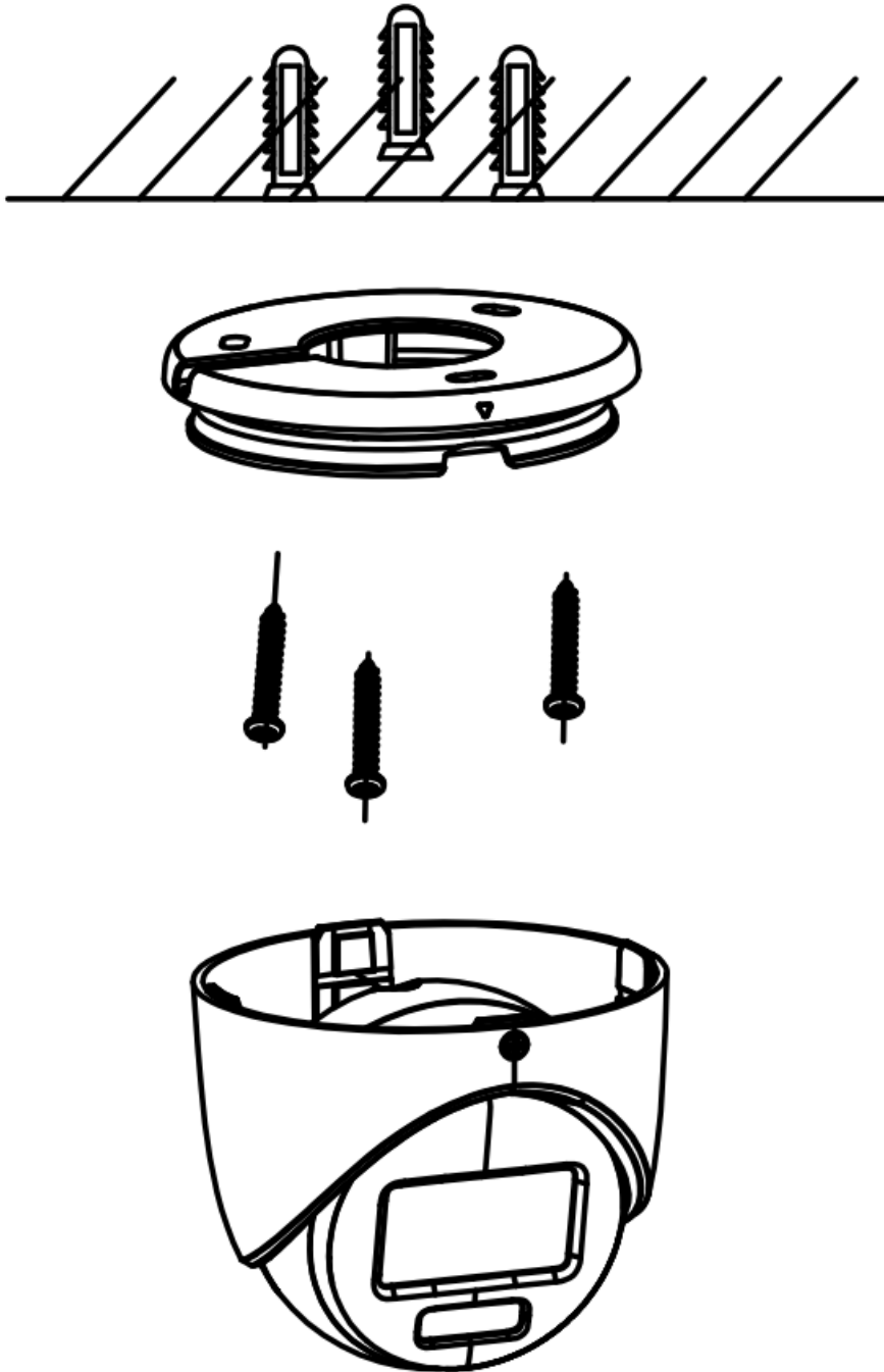
Figure 2-26 Install the Camera Back
