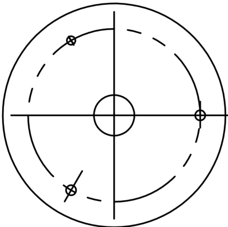
Figure 2-38 Drill Template
