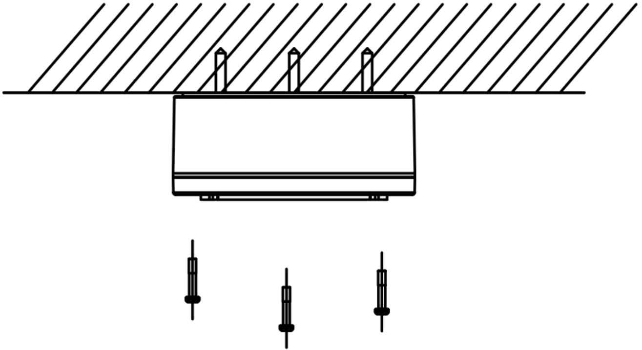
Figure 2-32 Fix the Base
