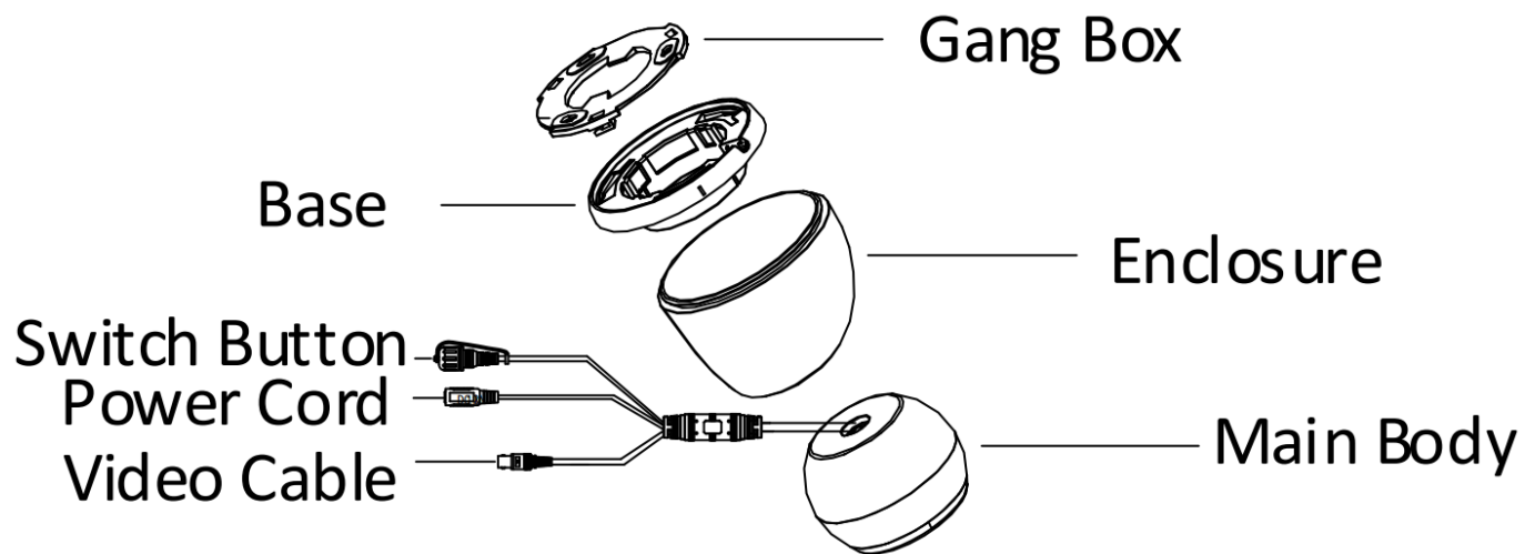
Figure 1-3 Overview of Type III Camera
