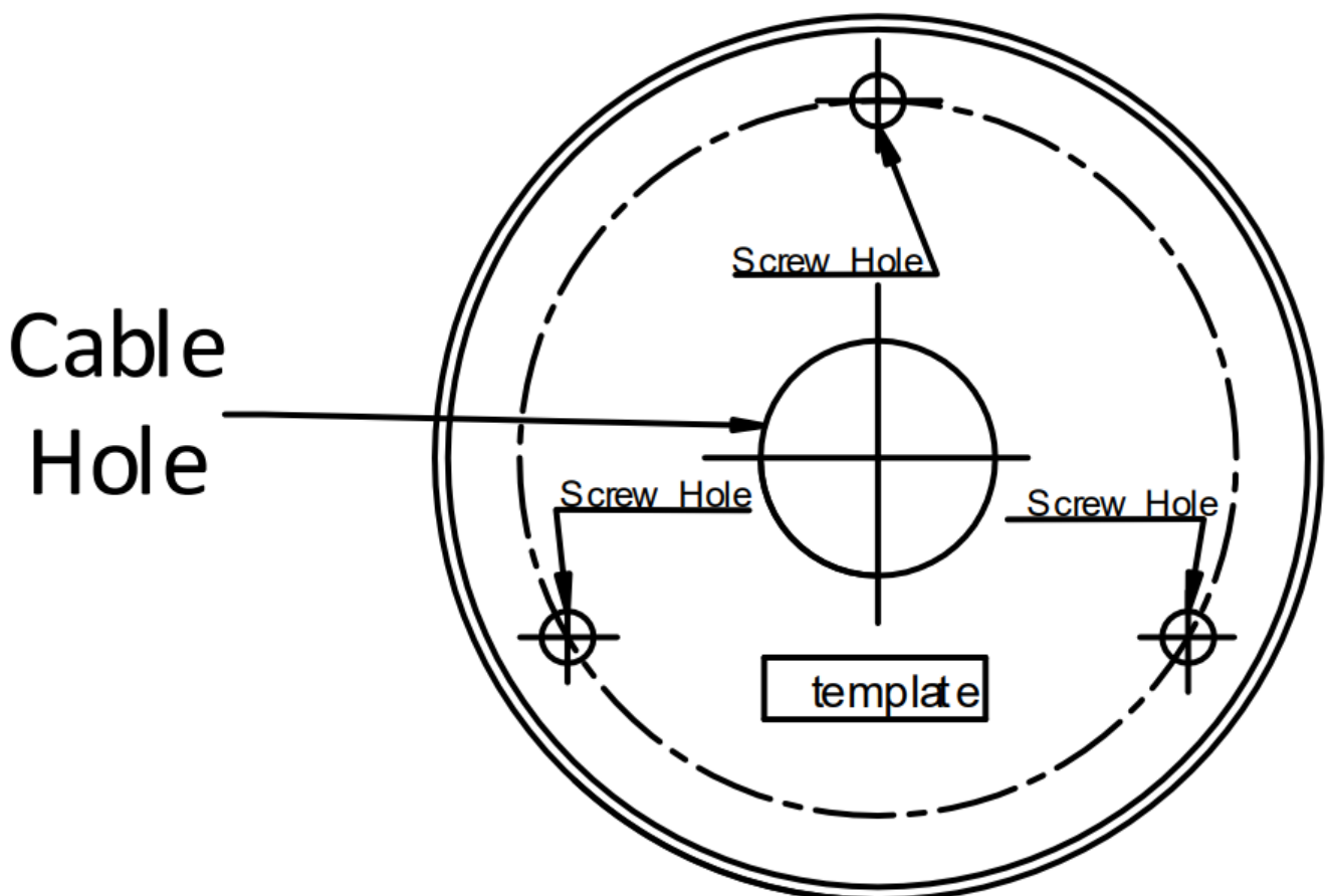
Figure 2-1 Drill Template
