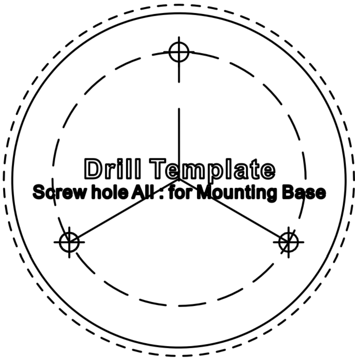
Figure 2-25 Secure the Base to the Ceiling
