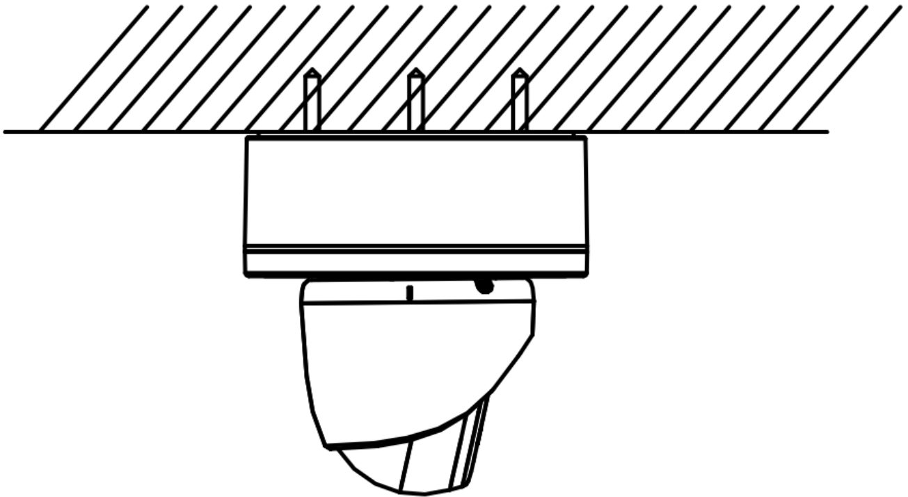
Figure 2-19 Finish the Installation
