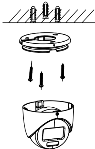
Figure 2-25 Secure the Base to the Ceiling
