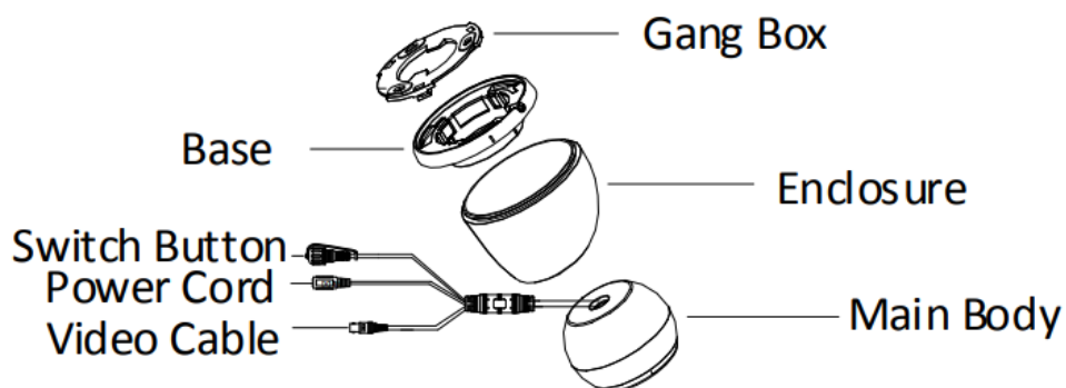
Figure 1-3 Overview of Type III Camera
