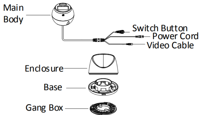
Figure 1-5 Overview of Type V Camera
