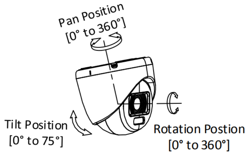
Figure 2-15 3-Axis Adjustment
