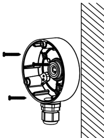
Figure 2-6 Secure the Junction Box on the Wall
