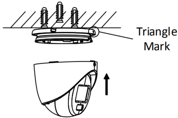
Figure 2-26 Install the Camera Back
