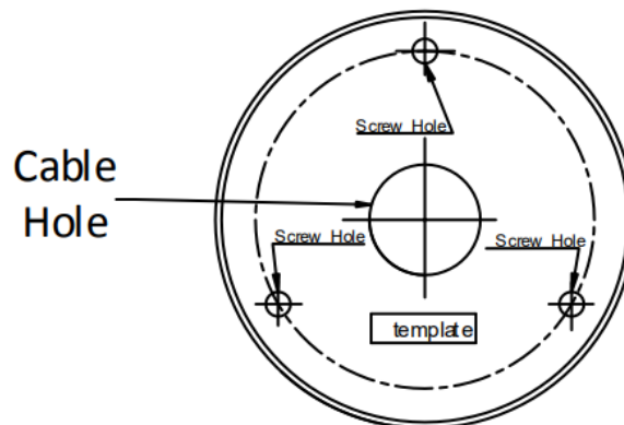
Figure 2-1 Drill Template
