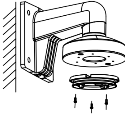
Figure 2-36 Fix the Wall Mount
