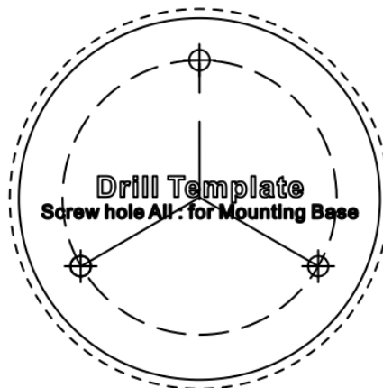
Figure 2-24 Drill Template
