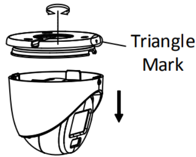
Figure 2-23 Disassemble the Camera
