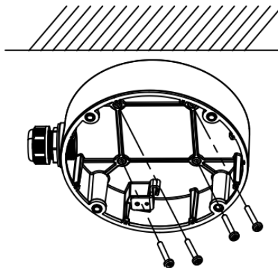
Figure 2-47 Secure the Junction Box Body
