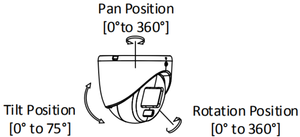
Figure 2-27 3-Axis Adjustment
