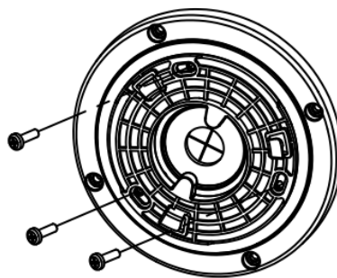
Figure 2-44 Install Gang Box to Junction Box Cover
