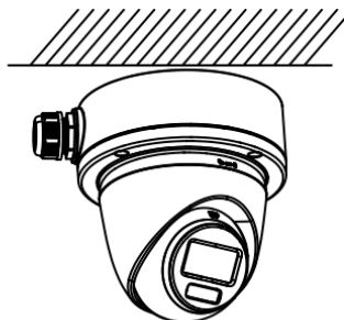
Figure 2-48 Combine Junction Box Cover with Body
