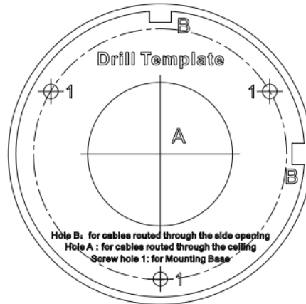
Figure 2-29 Drill Template for Junction Box
