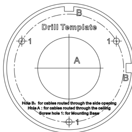
Figure 2-16 Drill Template for Junction Box
