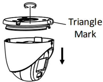
Figure 2-35 Disassemble the Camera
