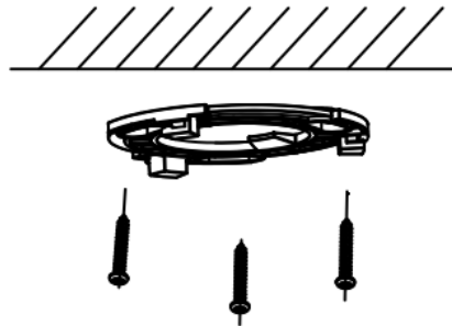
Figure 2-12 Attach the Gang Box to the Ceiling
