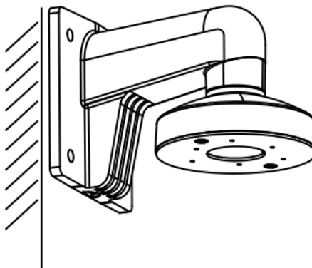
Figure 2-34 Fix the Wall Mount
