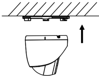
Figure 2-13 Fit the Camera onto the Gang Box
