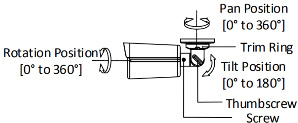
Figure 2-10 3-Axis Adjustment
