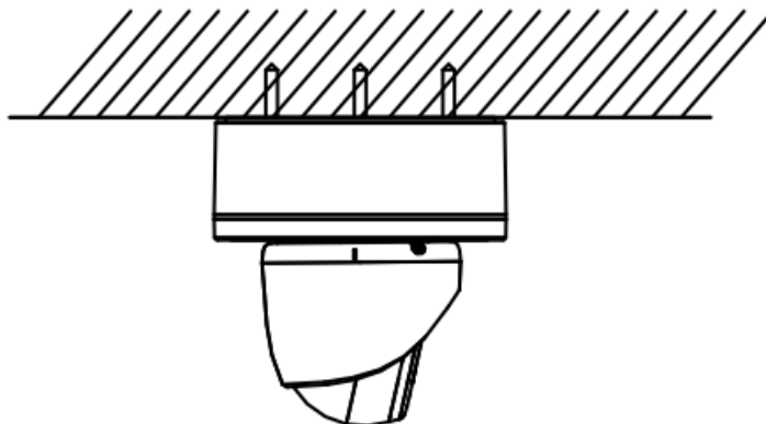
Figure 2-19 Finish the Installation
