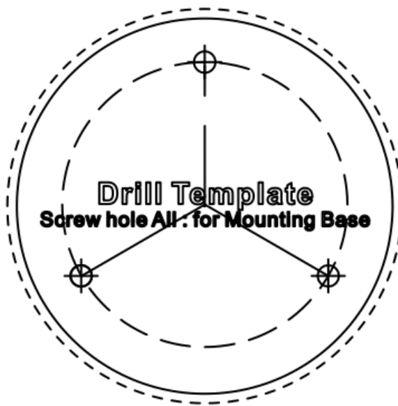
Figure 2-11 Drill Template
