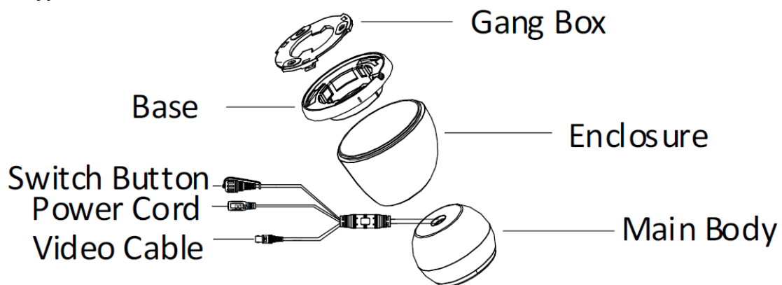
Figure 1-3 Overview of Type III Camera
