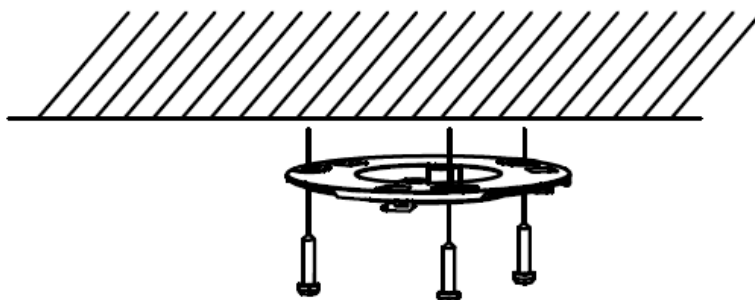
Figure 2-39 Attach the Gang Box to the Ceiling
