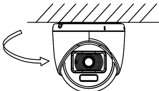
Figure 2-13 Fit the Camera onto the Gang Box
