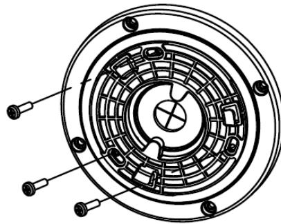
Figure 2-44 Install Gang Box to Junction Box Cover
