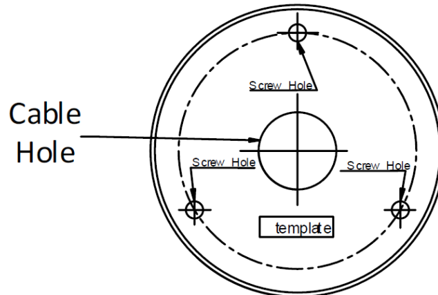
Figure 2-1 Drill Template
