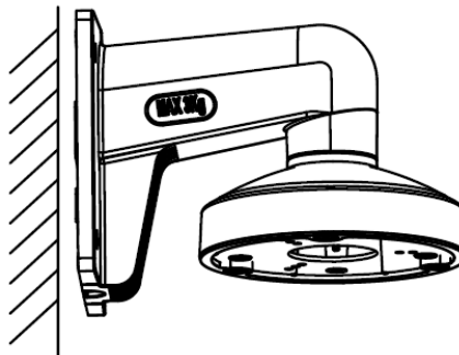
Figure 2-49 Fix the Wall Mount
