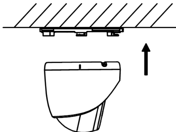
Figure 2-13 Fit the Camera onto the Gang Box
