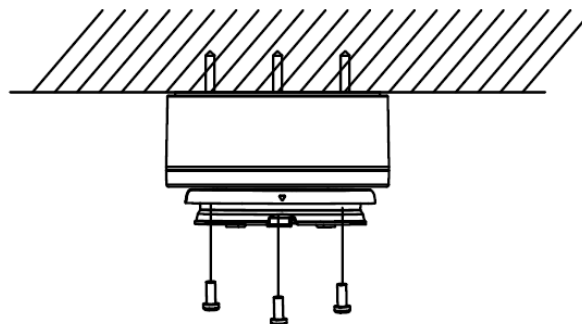
Figure 2-32 Fix the Base
