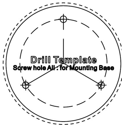
Figure 2-11 Drill Template
