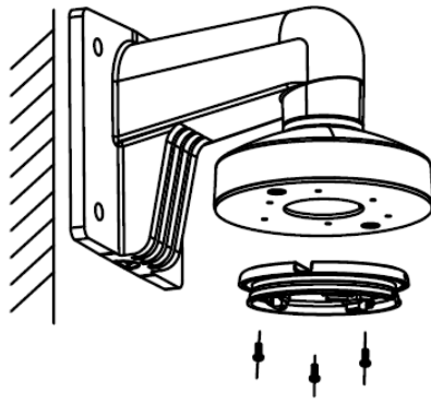
Figure 2-36 Fix the Base onto the Wall Mount
