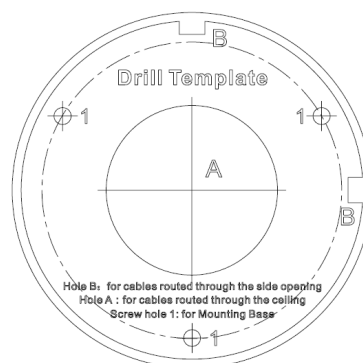
Figure 2-16 Drill Template for Junction Box
