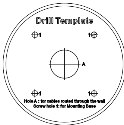
Figure 2-43 Drill Template
