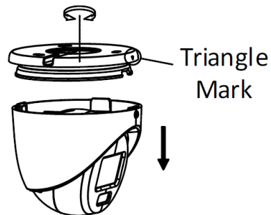
Figure 2-23 Disassemble the Camera
