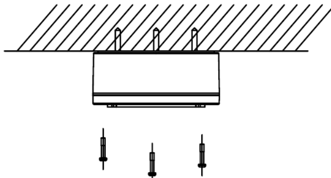
Figure 2-31 Combine the Junction Box Cover and Body
