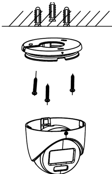
Figure 2-25 Secure the Base to the Ceiling
