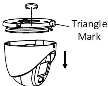
Figure 2-35 Disassemble the Camera
