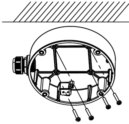
Figure 2-47 Secure the Junction Box Body
