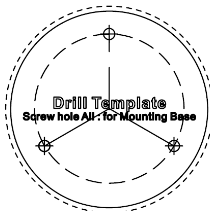
Figure 2-24 Drill Template
