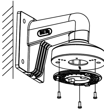
Figure 2-50 Fix the Gang Box
