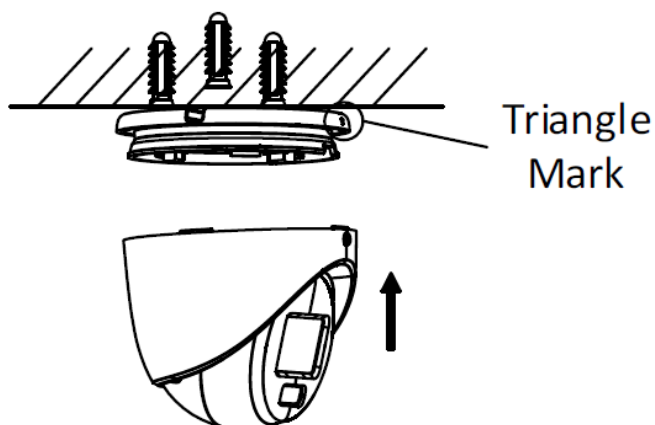
Figure 2-25 Secure the Base to the Ceiling
