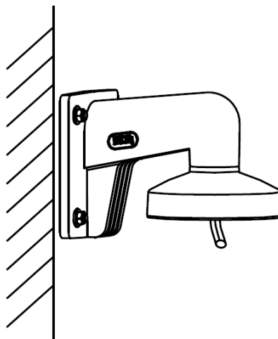
Figure 2-20 Fix the Wall Mount
