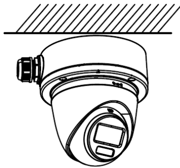
Figure 2-48 Combine Junction Box Cover with Body
