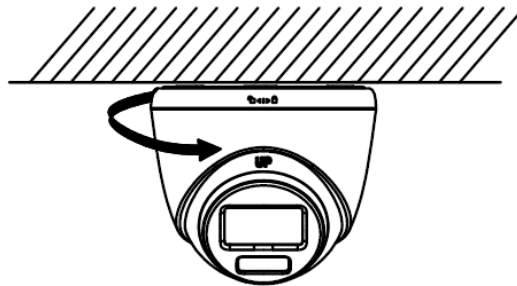
Figure 2-41 Snap the Camera into the Gang Box
