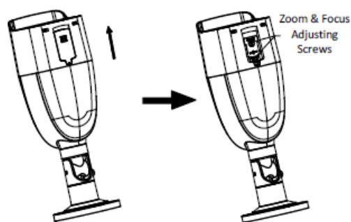
Figure 2-15 Remove Cover
