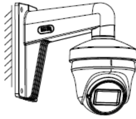
Figure 2-25 Finish Installation
