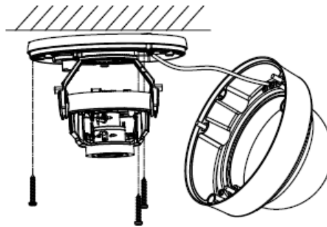
Figure 2-2 Install Mounting Base
