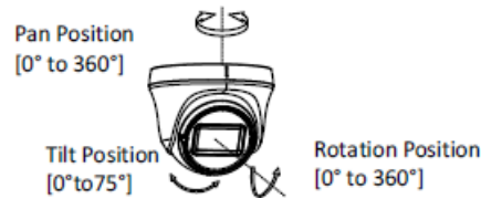
Figure 2-20 3-Axis Adjustment
