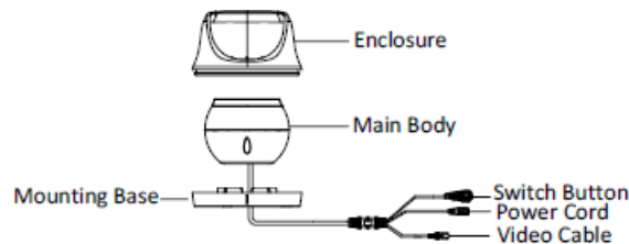
Figure 1-3 Overview of Type III Camera
