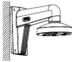
Figure 2-7 Install Bracket
