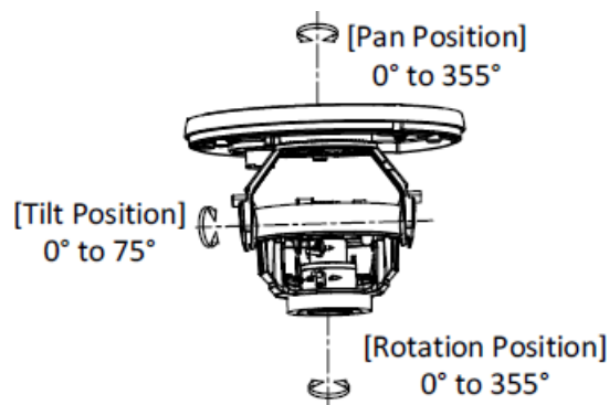
Figure 2-3 3-Axis Adjustment
