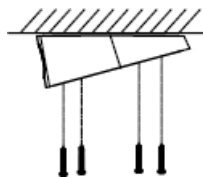
Figure 2-5 Install Inclined Ceiling Mount to Ceiling
