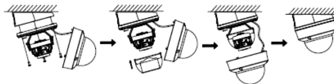
Figure 2-6 Fix Camera to Bracket
