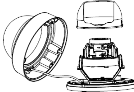
Figure 2-1 Remove Bubble and Black Liner
