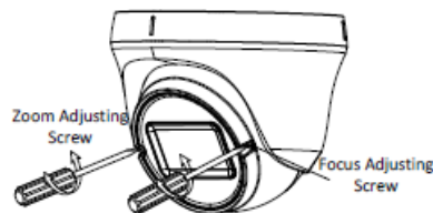
Figure 2-26 Adjust Zoom and Focus
