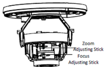
Figure 2-9 Adjust Zoom and Focus
