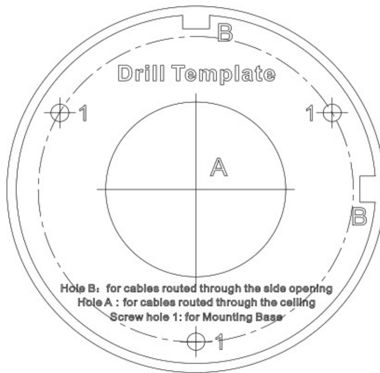
Figure 2-3 Drill Template for Junction Box
