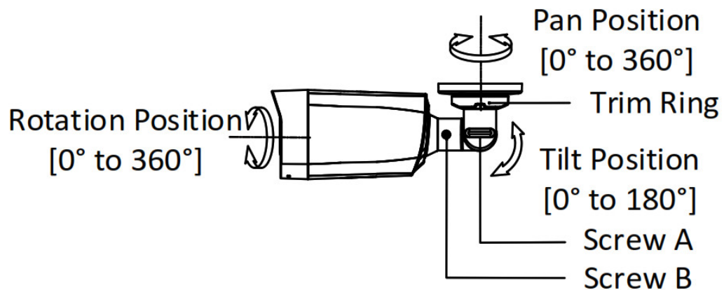
Figure 2-2 3-Axis Adjustment
