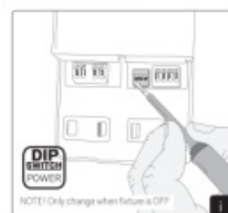
DIP on DALI driver
