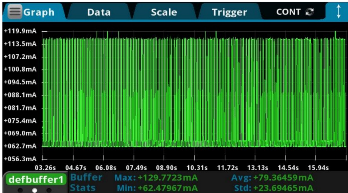
Figure 11 Measured data of module working current
