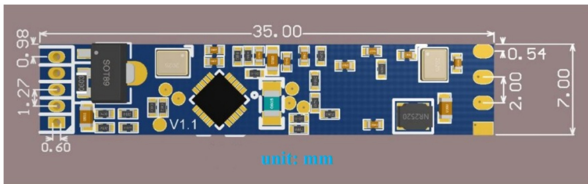
Figure 5 Module Dimensions
