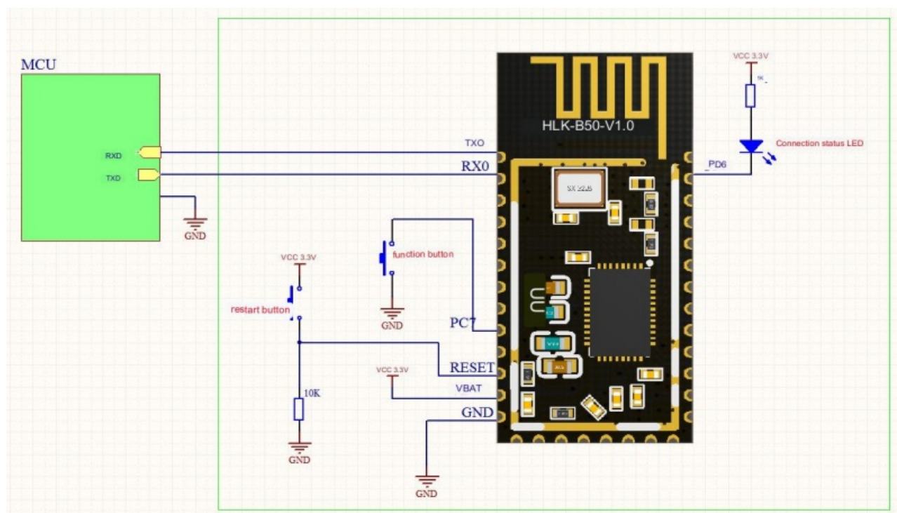
Figure 2 Basic minimum circuit
