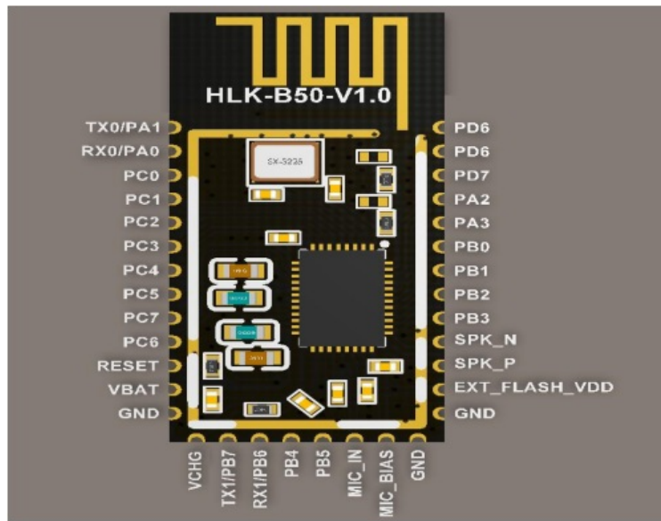
Figure 1 Pin location schematic
