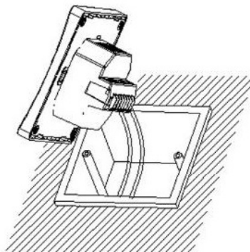
Connect the cables
