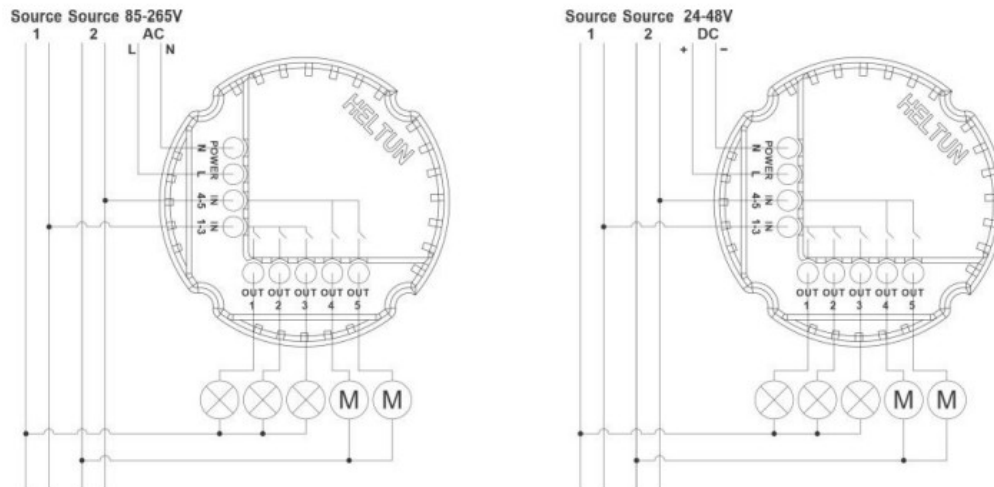
Figure 2: Connection Diagrams
