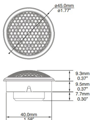
With housing for flush mount
