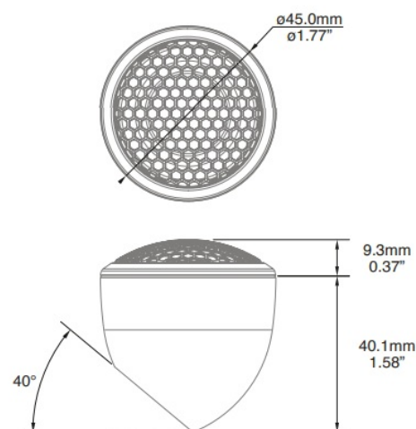
With housing for angle mount
