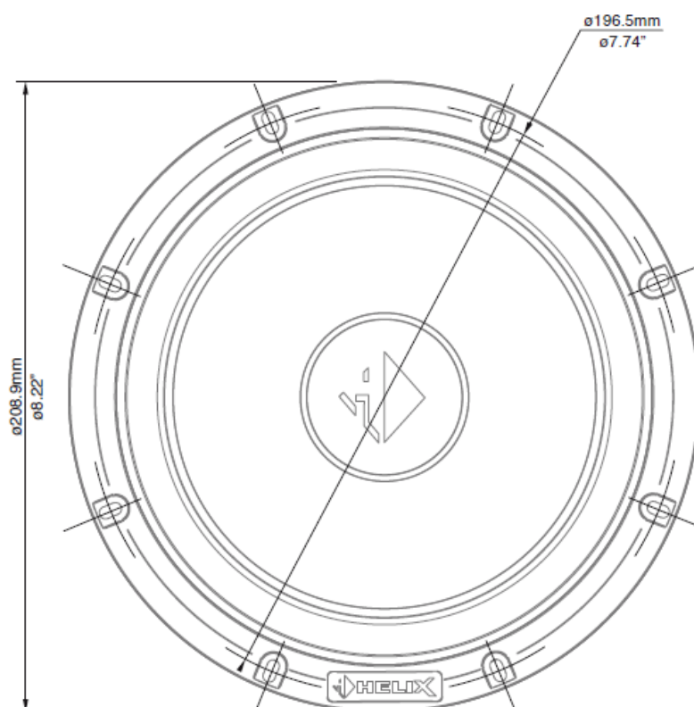
Woofer with assembled universal mounting ring
