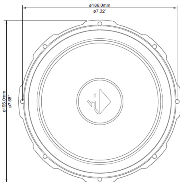
Woofer with assembled universal mounting ring
