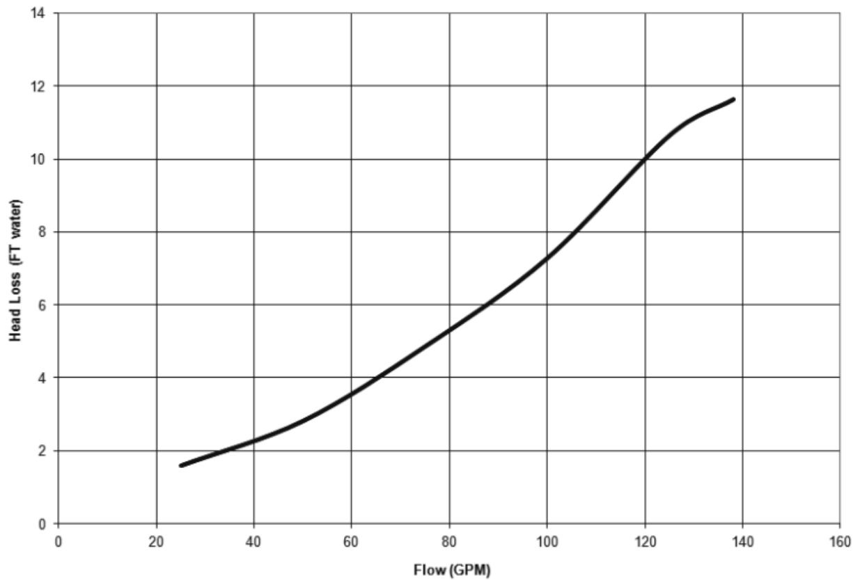
Head Loss Top Manifold
