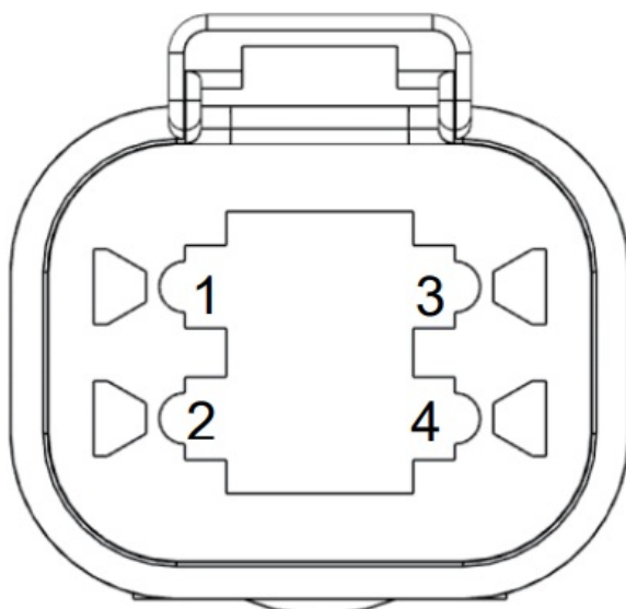
Power / Communication Tractor Harness 006-765IC at Baler Hitch (Deutsch Plug Number: HDP24-24-18PN)
