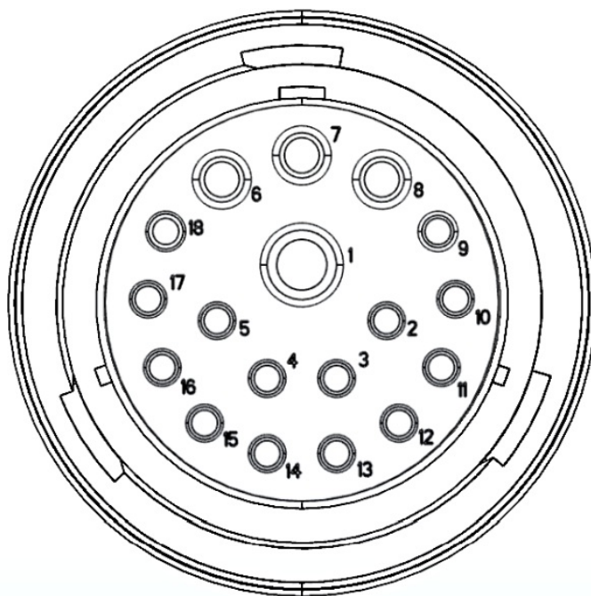
Power / Communication Baler Harness 006-765B2 at IPM Module (Deutsch Plug Number: HDP24-24-18SN)
