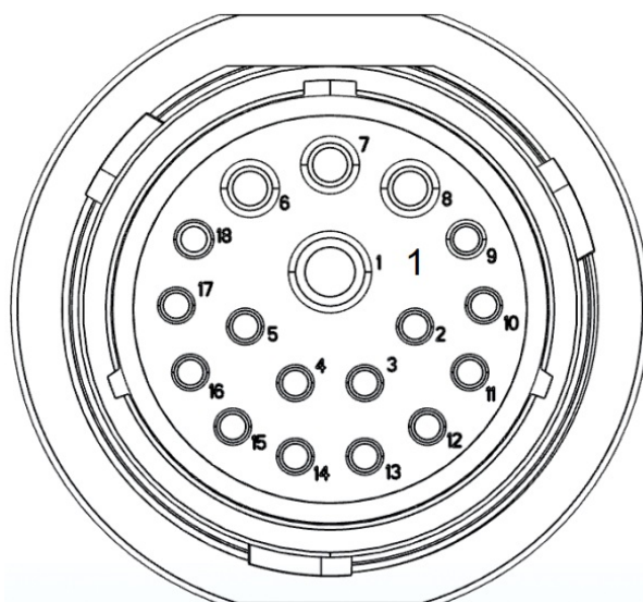
Power / Communication Baler Harness 006-765B2 at Baler Hitch IPM (Deutsch Plug Number: HDP26-24-18SN)
