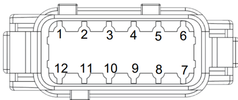
ISOBUS Plug on Tractor Harness 006-765IC (Deutsch Plug Number: DT04-4P)
