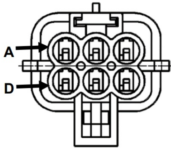
Pump Connection on 700 Controller Harness (16 AWG Two-Wire Plug)
