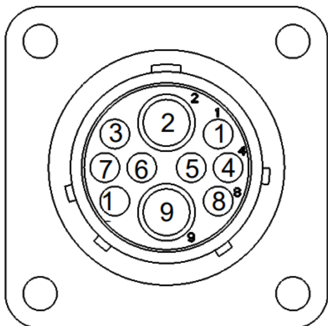
Power/Comm Harness 006-6650LS2(E) at Hitch
