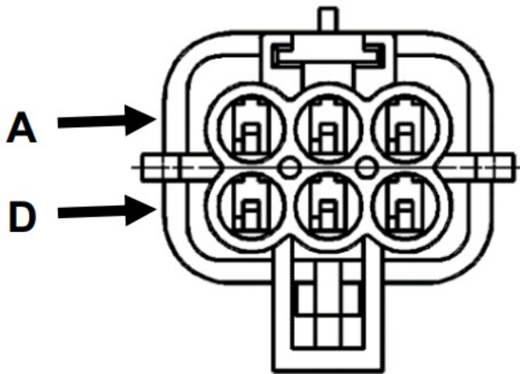
Main Power Connector on Dual Channel Processor (DCP)
