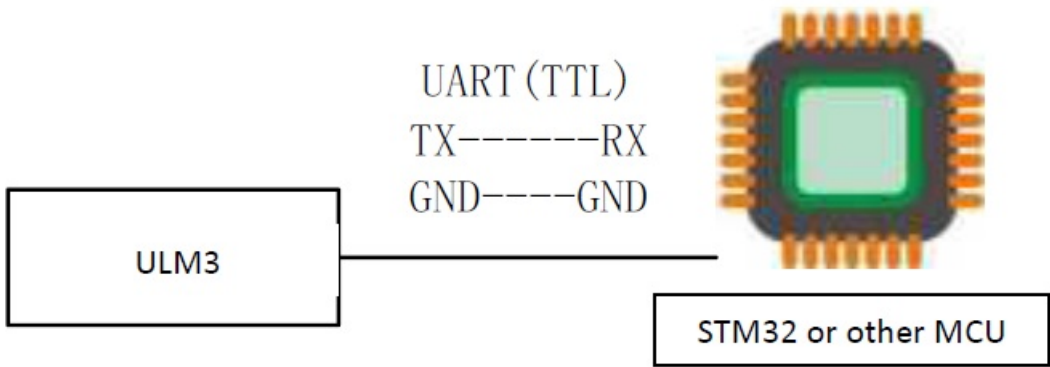
Figure 5-2 ULM3 UART Connection Diagram
