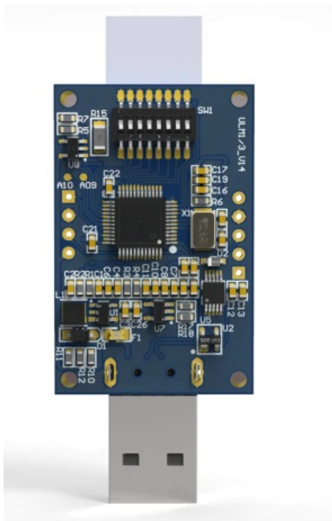
Figure 1-1 ULM3 UWB Module
