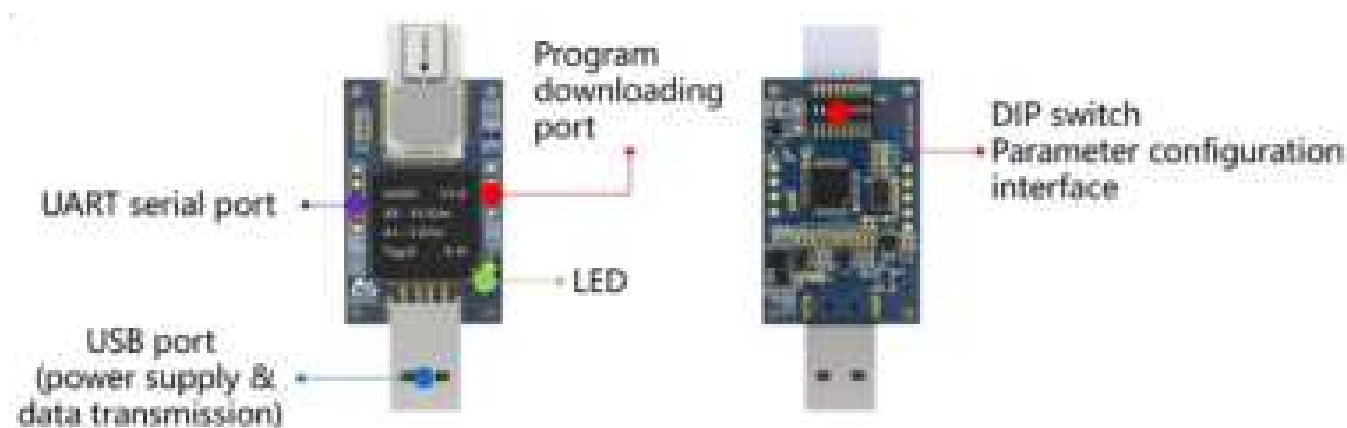
Figure 5-1 5-Module Interfaces
