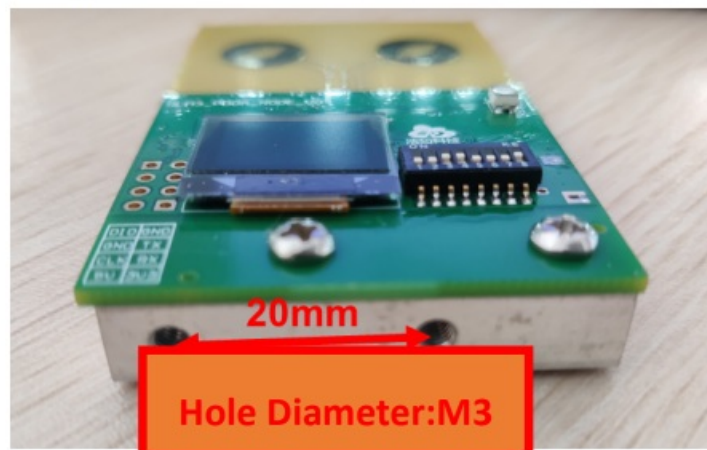
Figure 7-2 Mounting holes of bottom block
