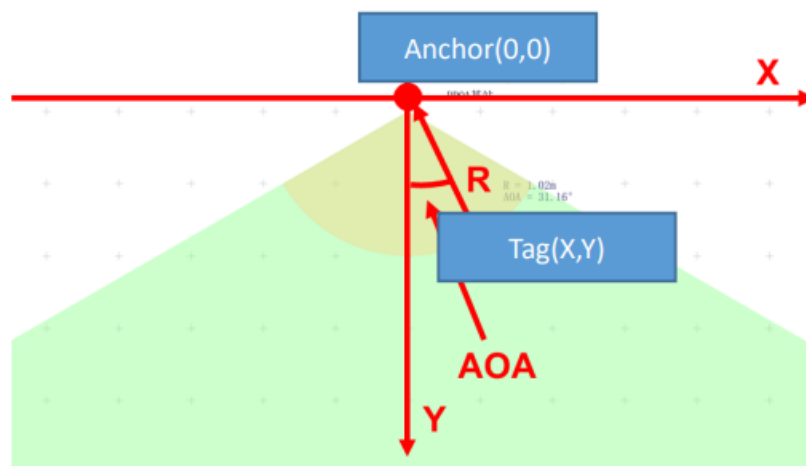
Figure 7-4 Positioning Range And Coordinate System
