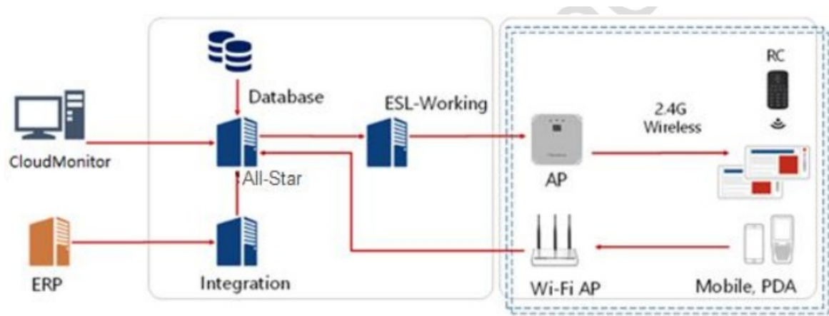
Figure 1-1 Hanshow ESL system architecture
