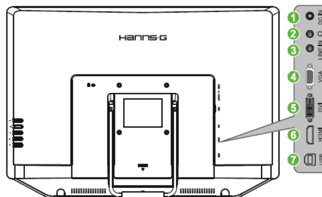
Figure.2. Connecting to a PC
