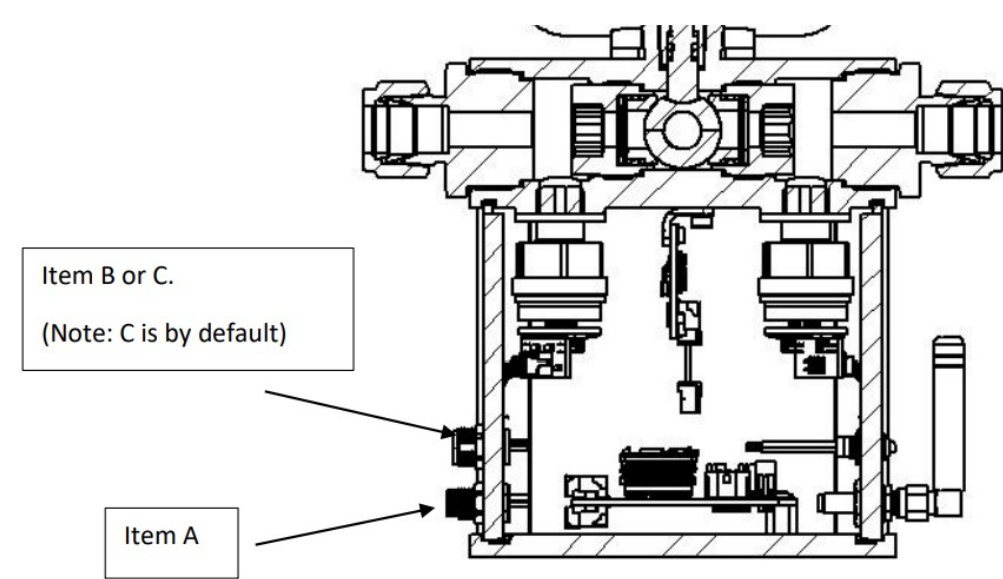
M8 4pins Female with Loose Wire (DC Supply & Mod-Bus Control)
