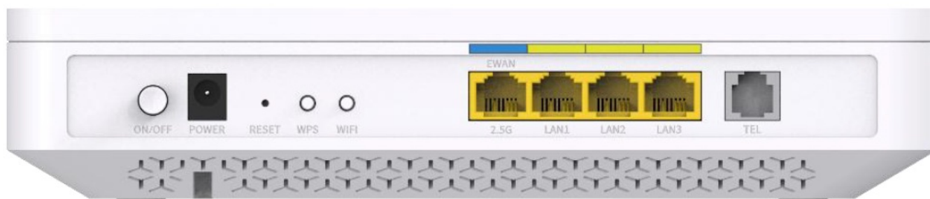
Fig2. Rear Panel
