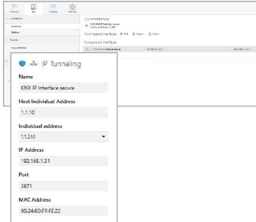
Figure 9 – IP Tunneling
