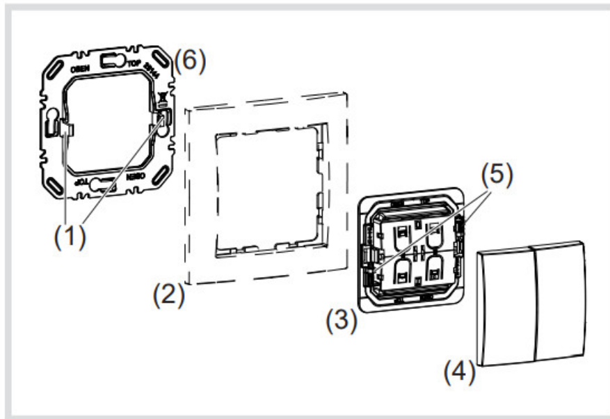
Image 1: Fundamental design and layout of the device
