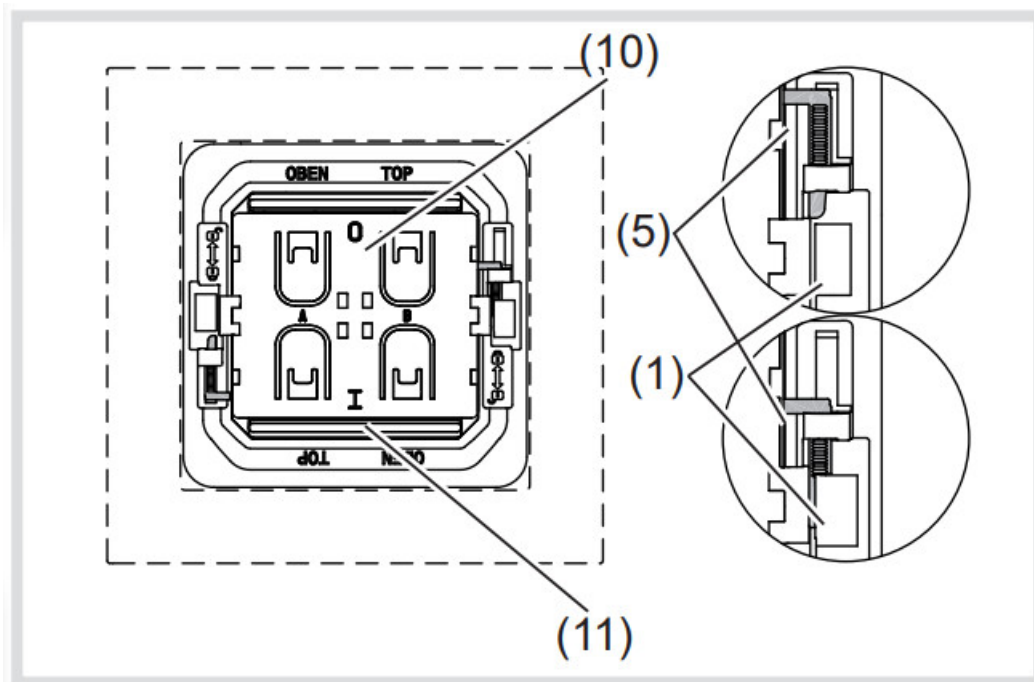
Image 4: Locked and unlocked Berker push-button Dismantling the device
