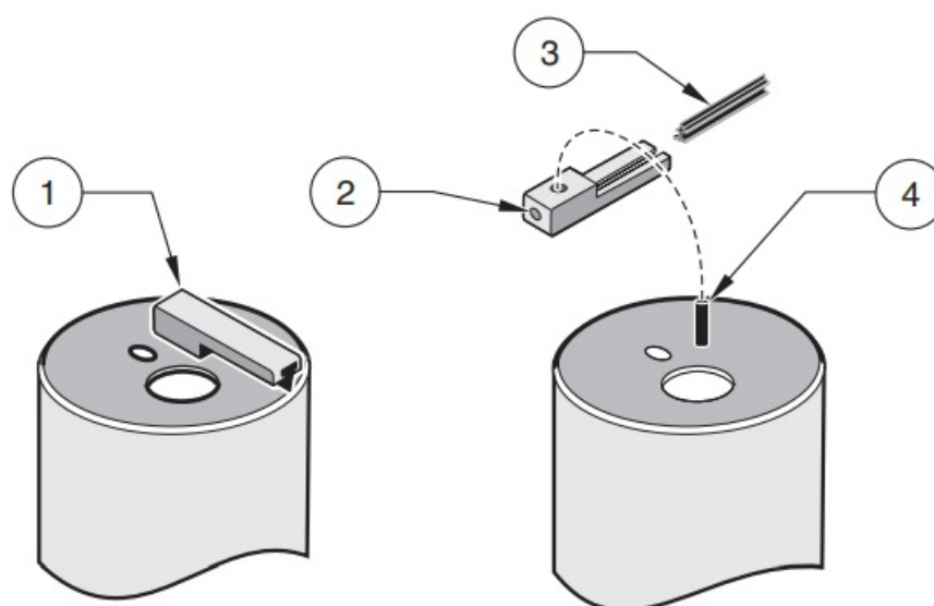
Figure 8 Wiper Replacement
