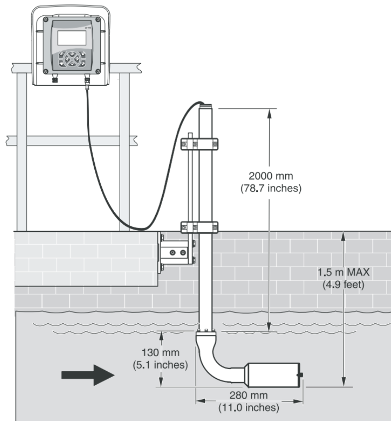
Figure 4 Sensor Installation Overview
