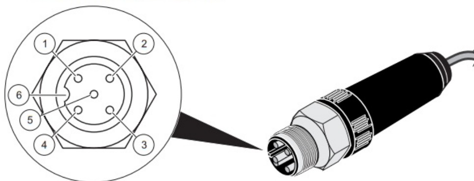
Figure 7 Sensor connector pin assignment
