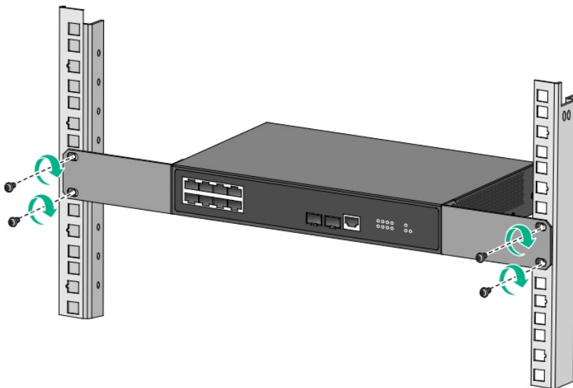
Figure2-7 Mounting an S1850V2-10P-EI switch in the rack
