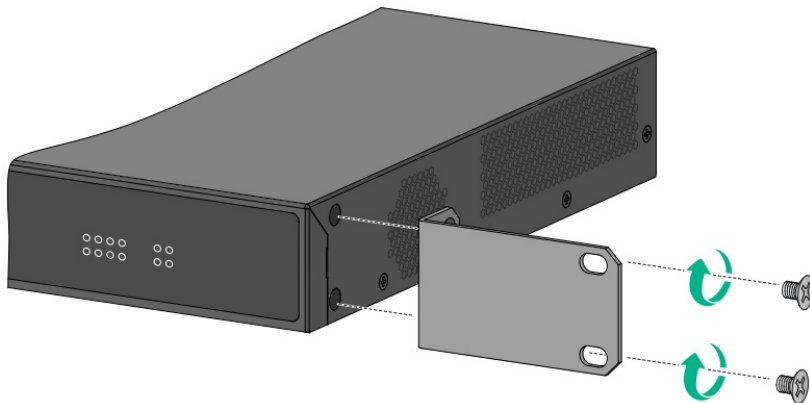
Figure2-5 Attaching mounting bracket C (S1850V2-10P-EI switch)
