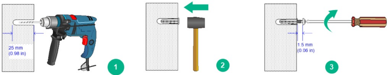
Figure2-10 Installing the switch on a wall (2)
