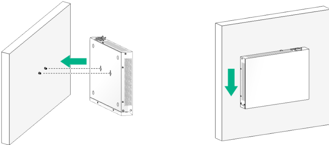
Figure2-11 Installing the switch on a wall (3)
