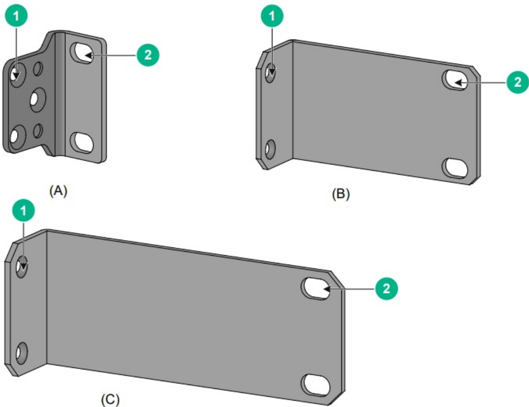
Figure2-2 Mounting brackets
