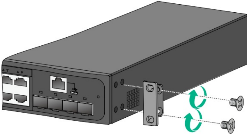
Figure2-4 Attaching mounting bracket B (S1850V2-10P-PWR-EI switch)
