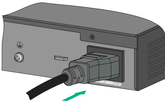
Figure2-16 Securing the AC power cord for the fixed AC power supply through a cable tie (S1850-52X switch)
