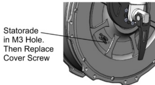
Figure 11: Statorade Fill Port.
