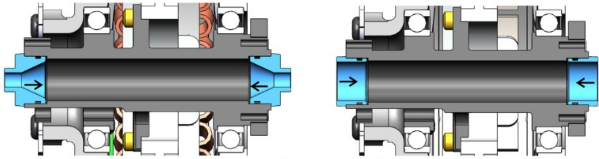
Figure 7: Example of quick release (left) and thru-axle (right) end caps, slid into place. In most adapter kits the left and right caps are identical.
