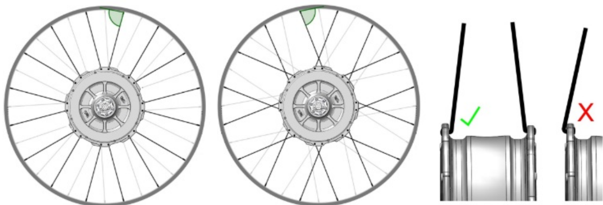
Figure 12: 0 Cross (left) is recommended, but for 24" and larger 1 cross (middle) is OK too. Even if dishing optimization suggests otherwise, lace both left and right side spokes with elbows in.
