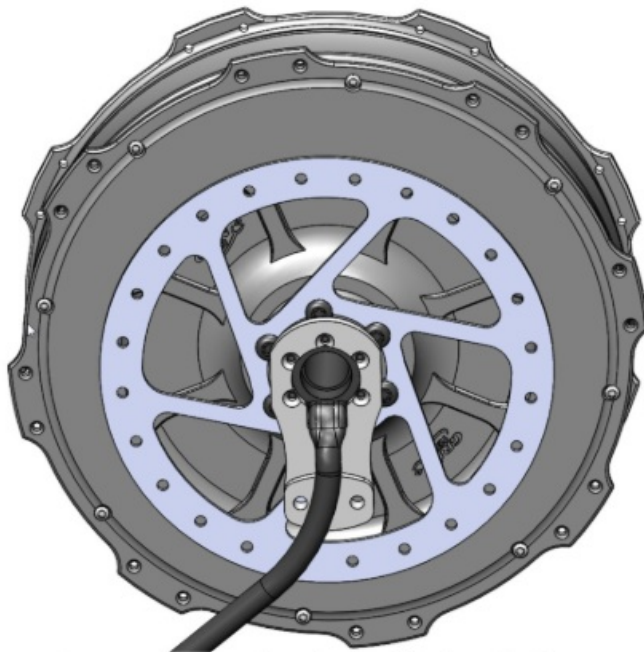
Figure 14: Torque Arm for single side installations on same side as cable and disc rotor.
