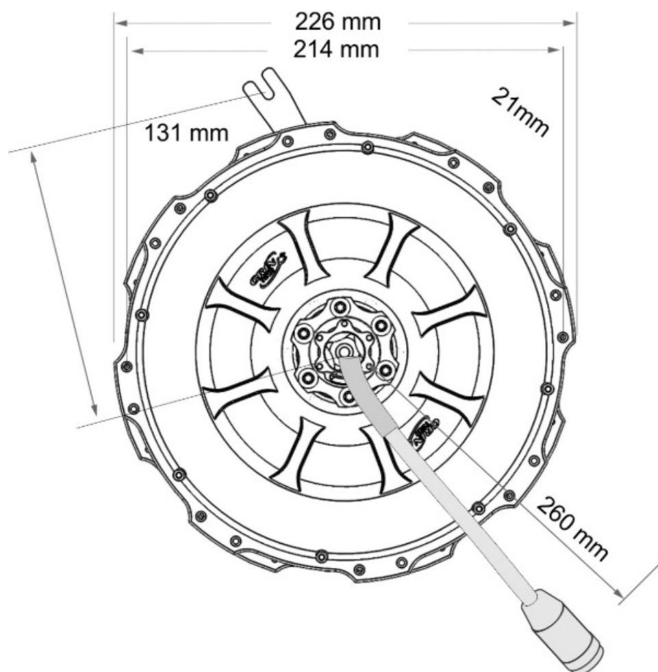
Figure 15: Mechanical Drawing
