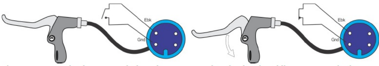
Figure 7: Most Ebrakes are switches that connect the ebrake signal line to ground when the brake lever is pressed. Pinout shown is from male connector perspective.
