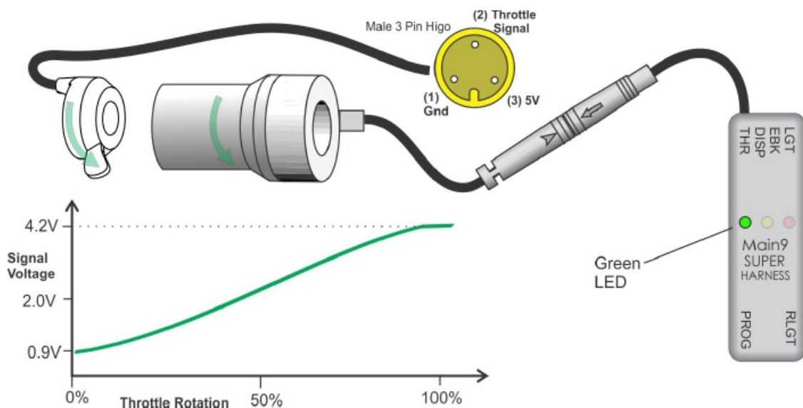
Figure 5: Signal output of a typical throttle. Green LED increases in brightness with throttle position. Pinout shows male throttle side Higo connector.
