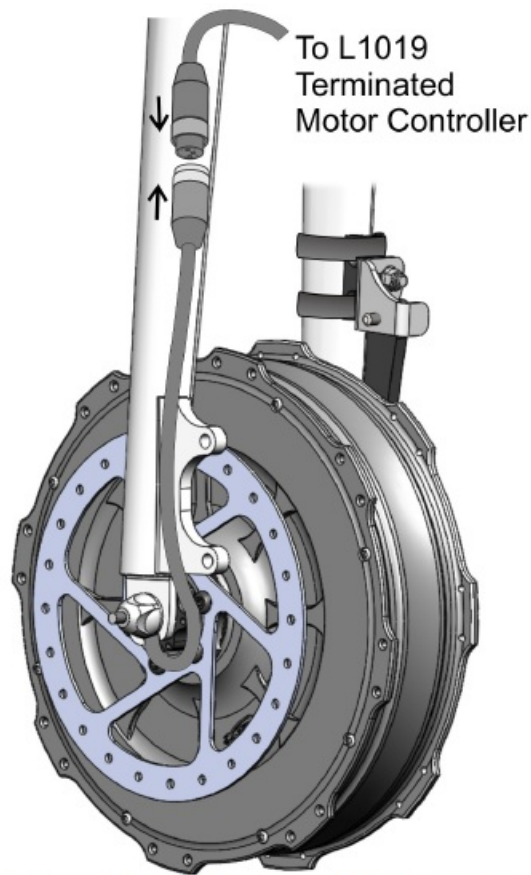
Figure 10: Cable will usually be held snug to fork with zip ties.
