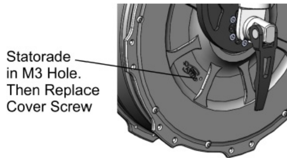
Figure 11: Statorade Fill Port.
