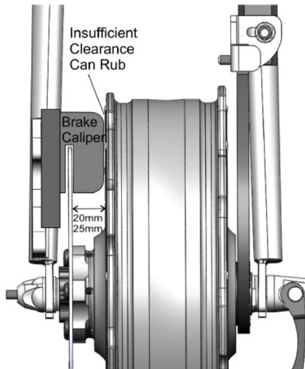
Figure 13: Illustration of Caliper Clearance.
