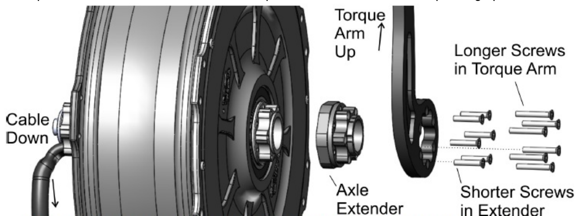
Figure 5: The torque arm screws should include a drop of threadlocker on the threads. Tighten with T10 Torx wrench (included) to 1 Nm.
