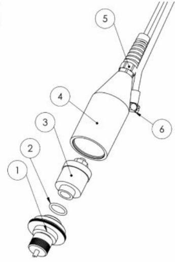
GOG / ResOx 5695 housing
