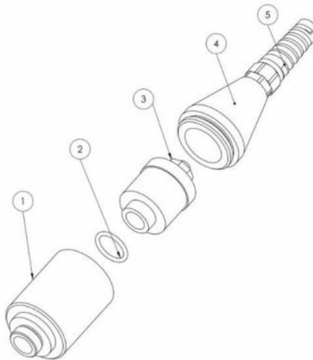
GGO/GGA housing
