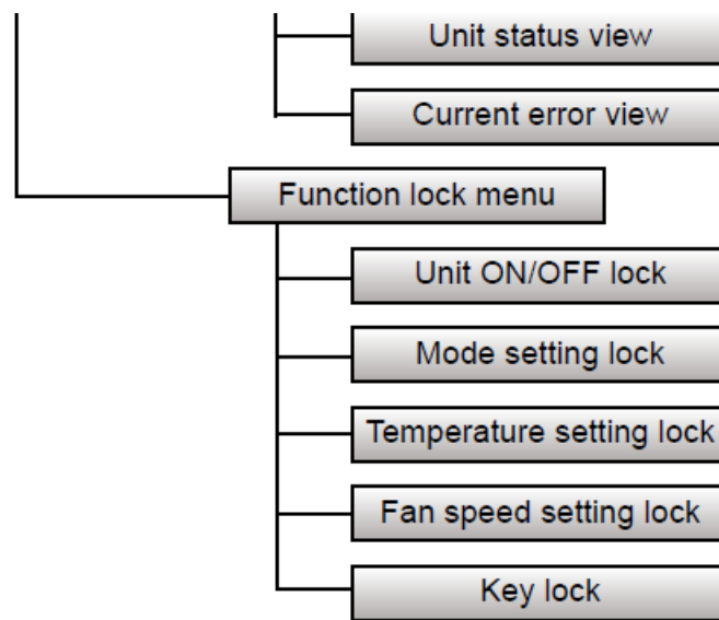
Fig. 3 Menu structure
