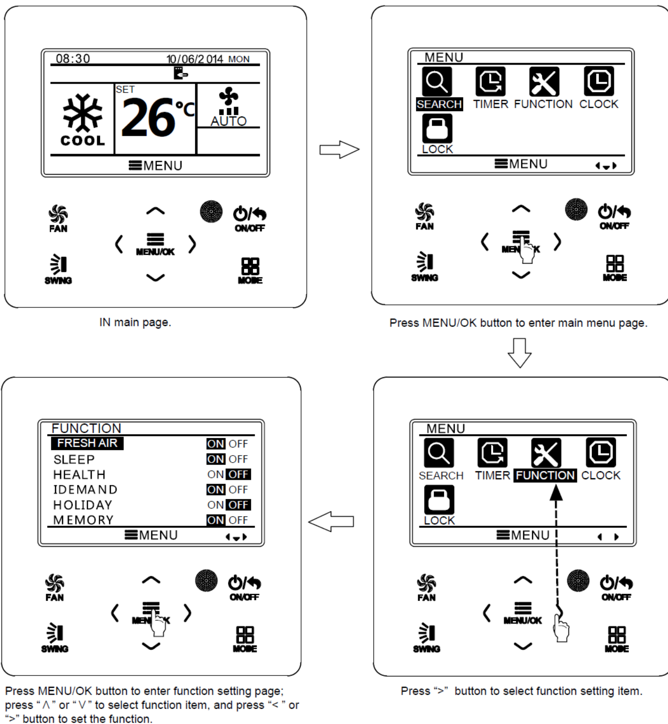
Fig. 8 Function setting
