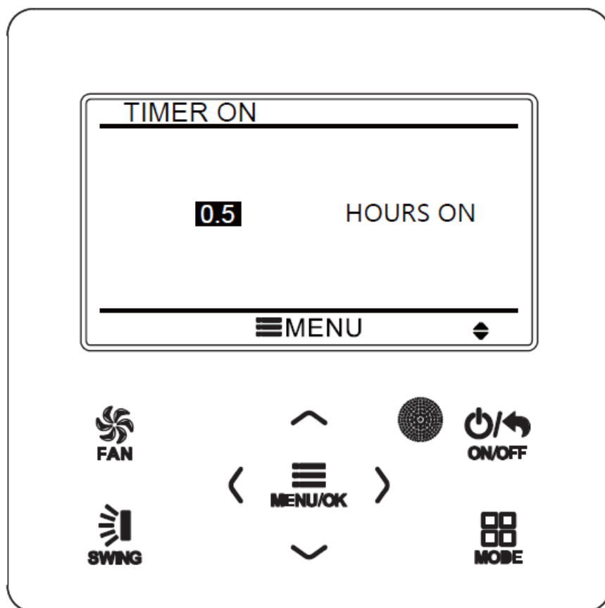
Fig. 16 Countdown timer on
