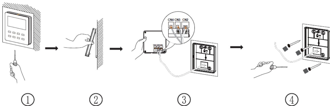
Fig. 24 Disassembly diagram for wired controller
