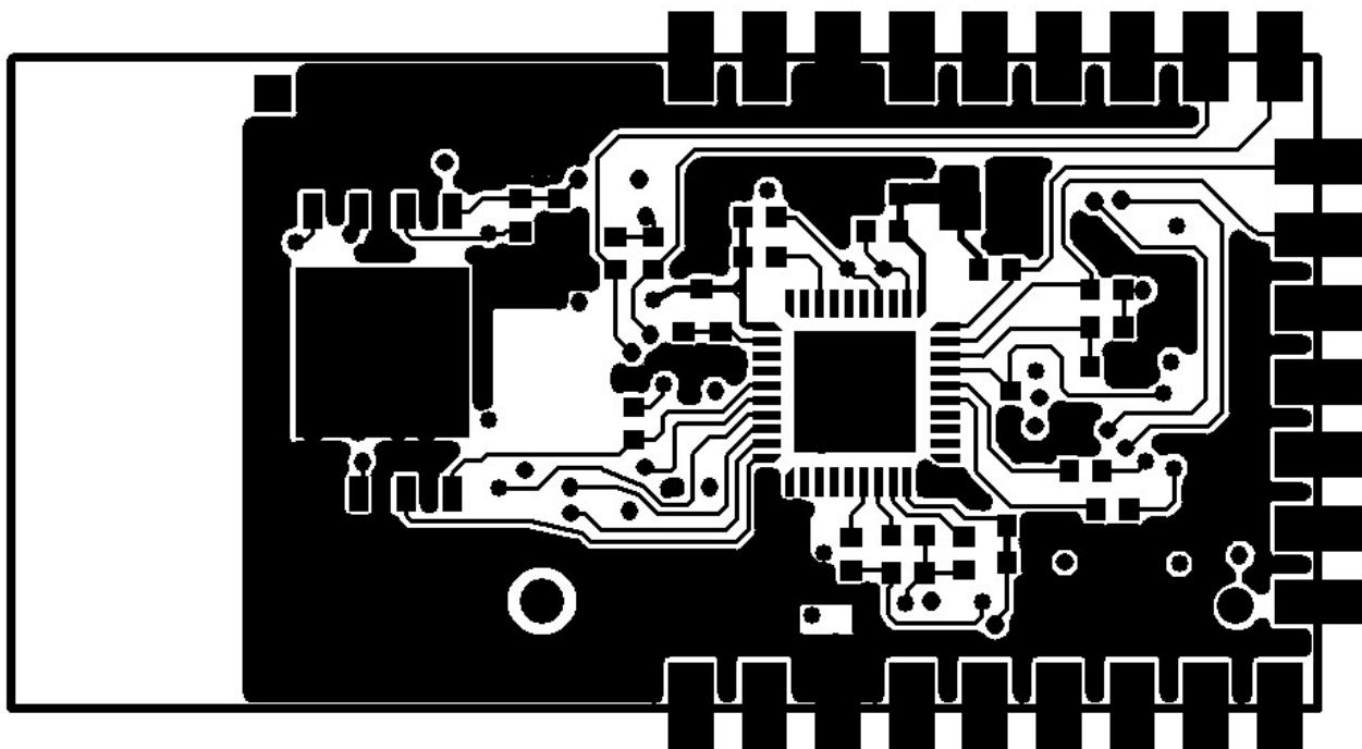
Silkscreen Bottom
