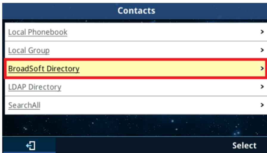
Figure 4: Contact Page
