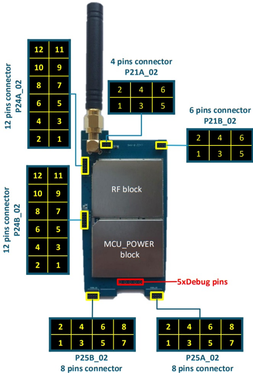
Figure 2-2 Frontside of board
