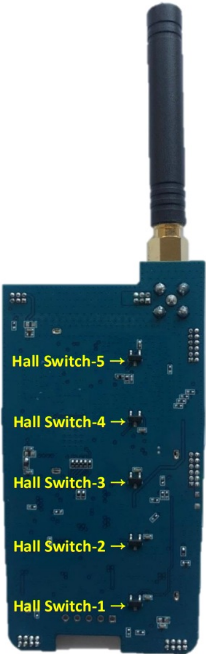
Figure 2-3 Backside of board
