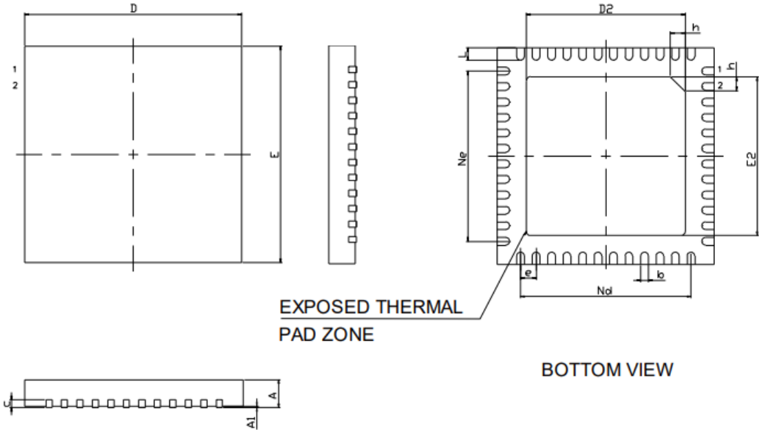
Figure 4-1 Package Outline QN48
