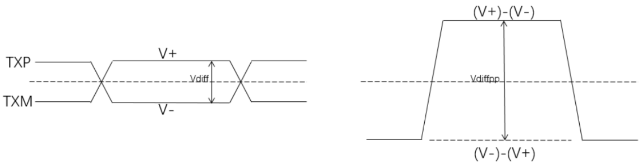
Figure 3-6 Transmit Differential Signal Swing V_{diffpp}
