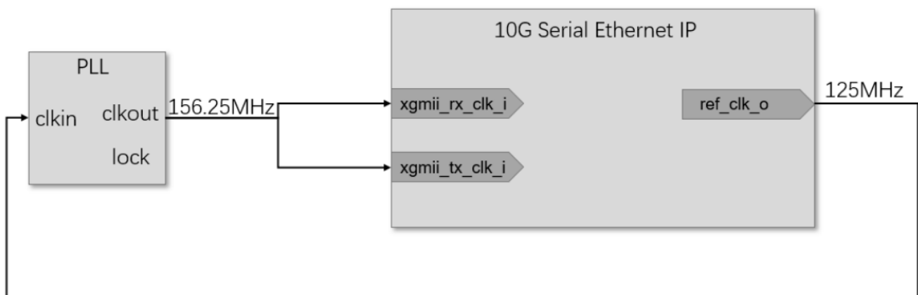
Figure 3-5 Clock Connection Reference (ref_clk_o outputs a clock with 125MHz)
