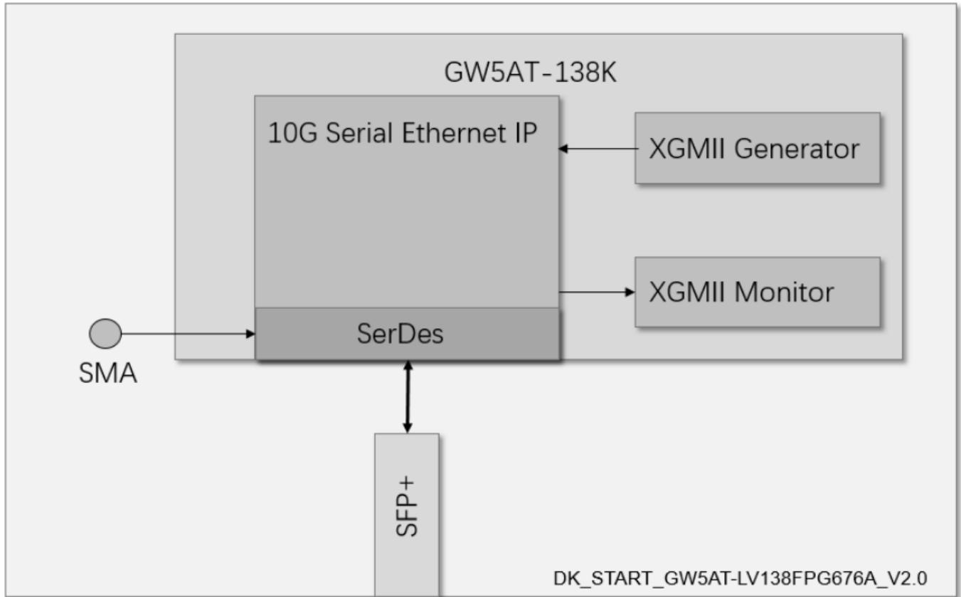
Figure 7-1 Hardware Platform and Diagram
