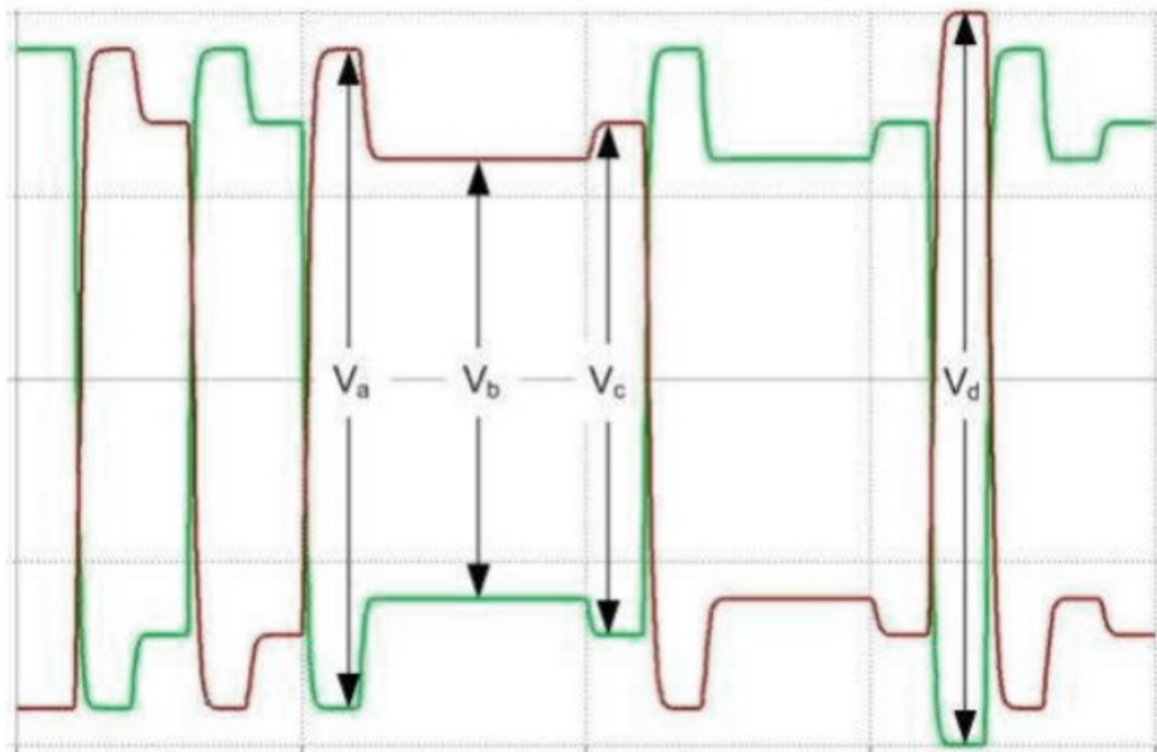
Figure 3-7 Voltage Definition for FFE TX
