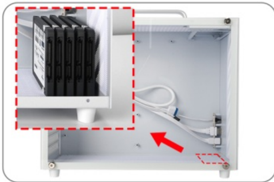
HDD Installation Location (Support up to 2.5" HDD *5)
