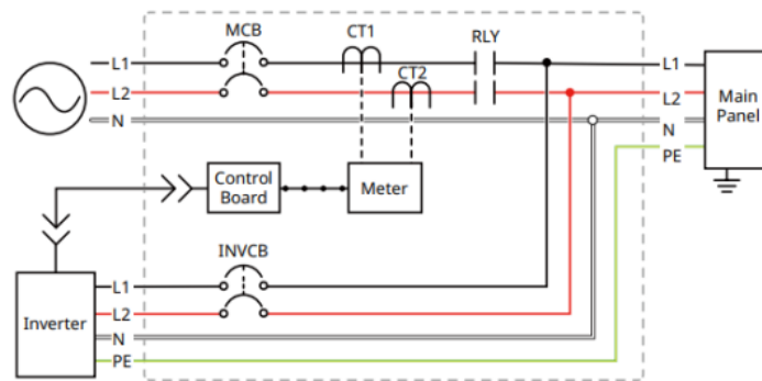
2.3.2 Electrical Diagram – MPD
