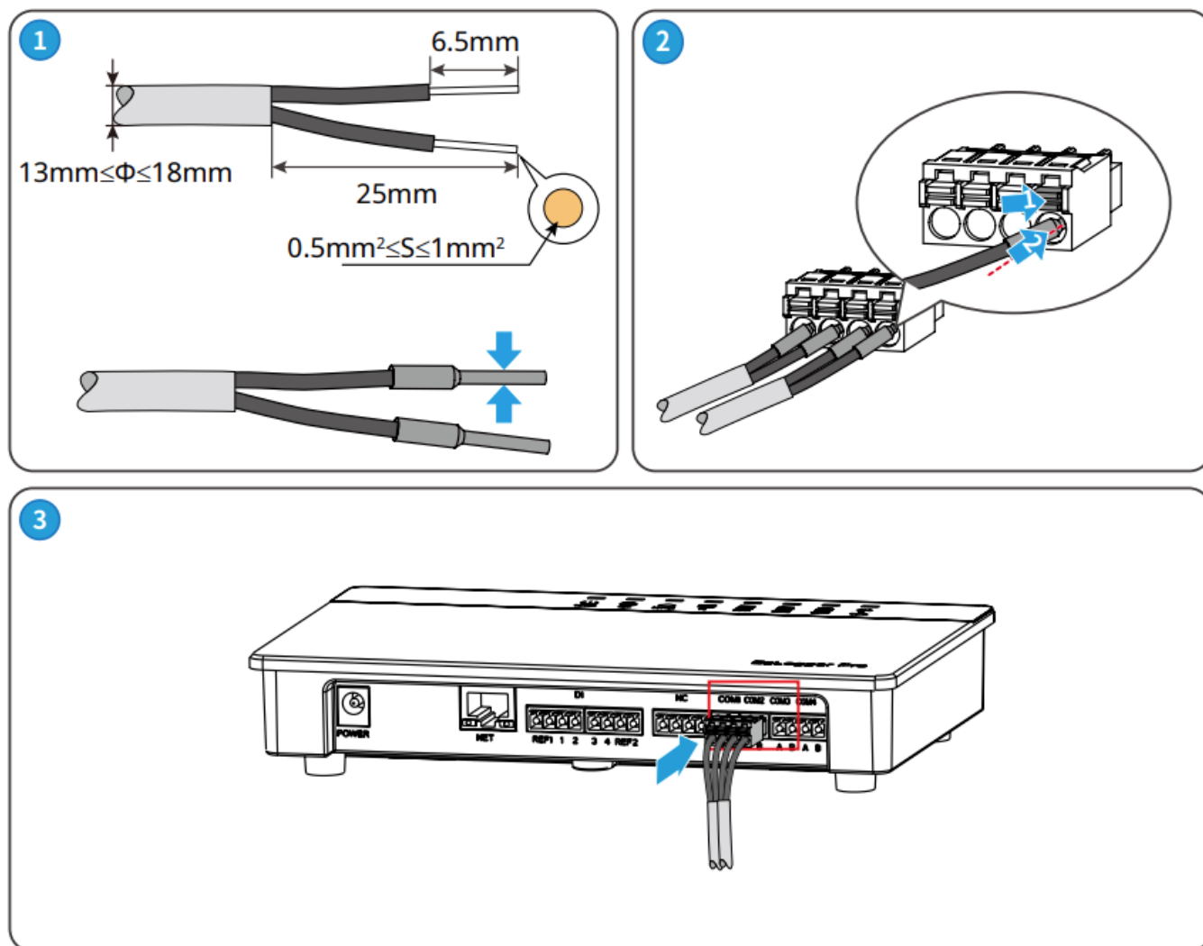
Figure 4.2.1-3 Wiring of EzLogger Pro COM port
