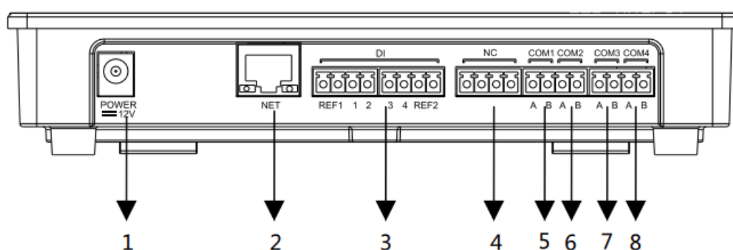
Figure 2.2-6 Bottom View of EzLogger Pro Box
