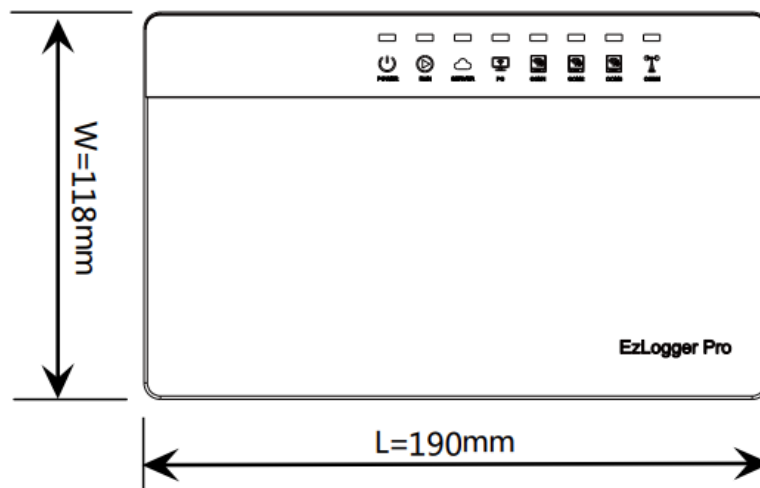
Figure 2.2-2 Front View of EzLogger Pro Box
