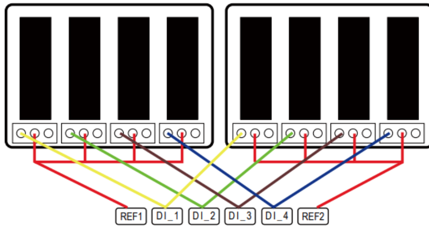
Figure 4.4-2 Diagram of Connection of EzLogger Pro DI Port to RCR
