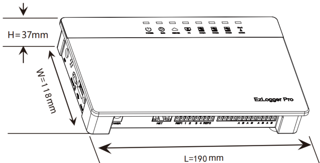
Figure 2.2-1 External View of EzLogger Pro
