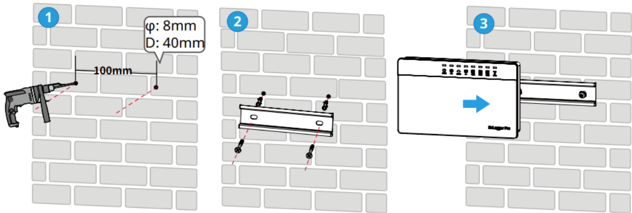
Figure 3.2.2-2 Schematic Diagram of Rail Mounting
