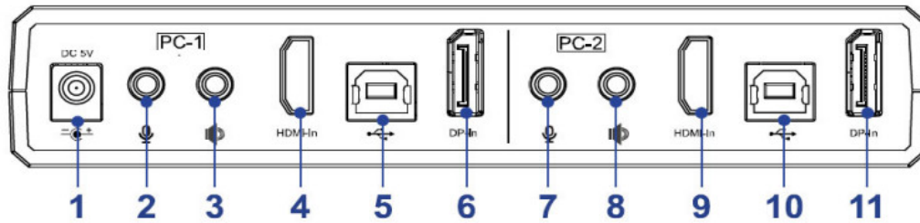
Figure 2: Rear Panel Layout
