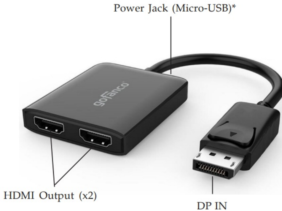
Figure 1: Layout
