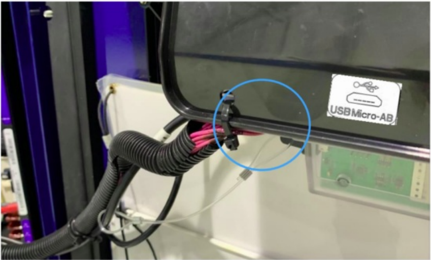
Figure 7c: Routing wire harness and label location
