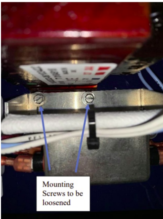
Figure 6b: Filter mounting screw
