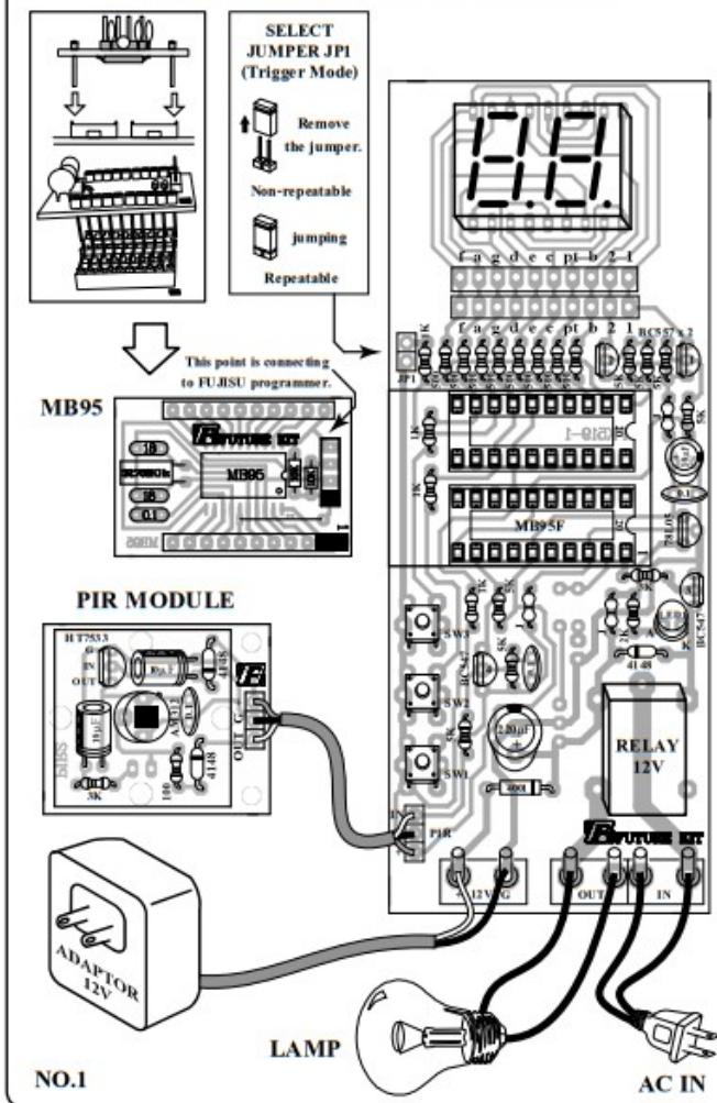
Figure 2. Circuit Assembling
