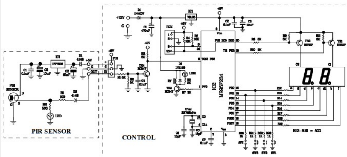
Figure 1. The PIR Motion Sensor With Timer Circuit
