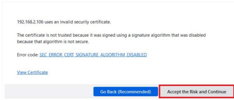
Figure 3: HTTPS confirmation
