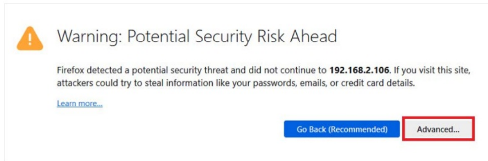
Figure 2: HTTPS input
