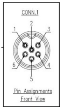
Pin assignments
