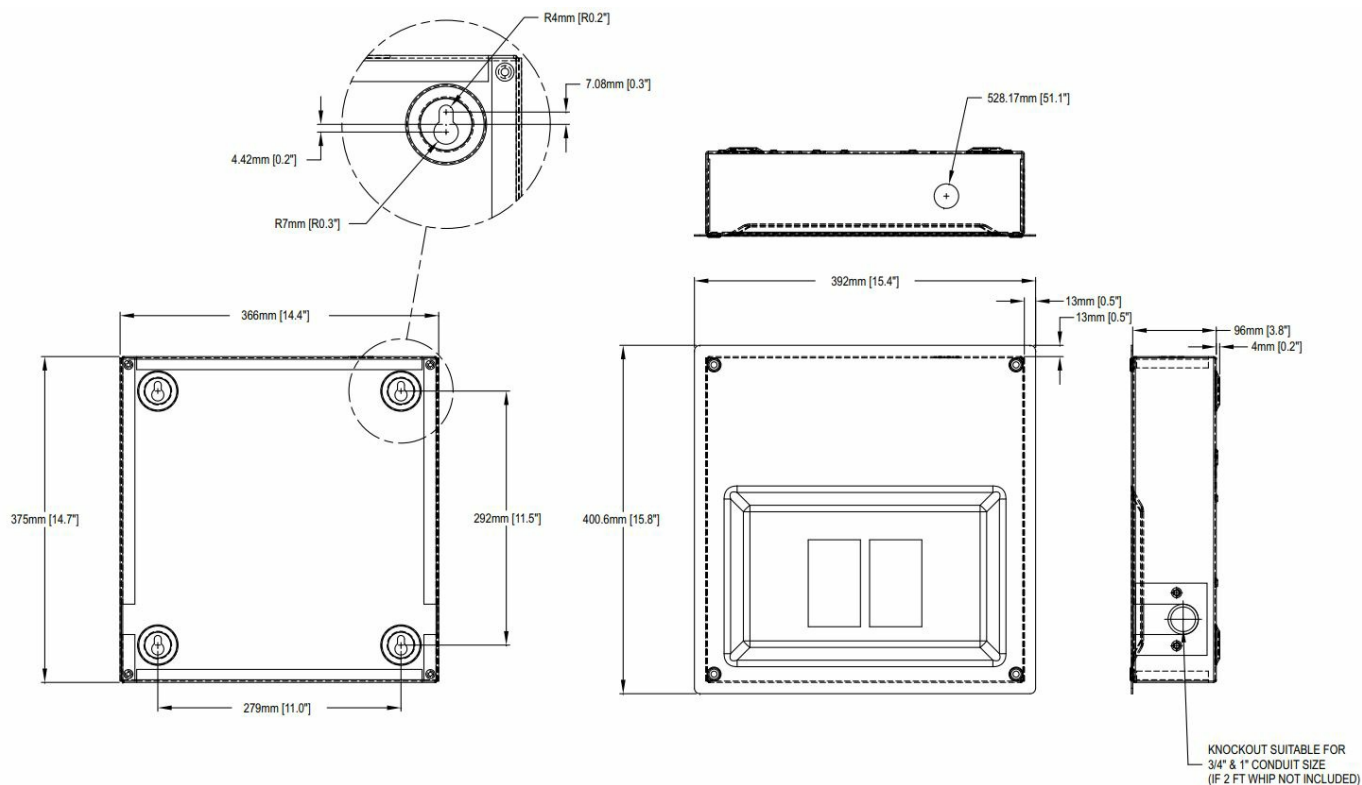
Interconnection Drawing No. 0K8845-A (Manual Transfer Connections)
