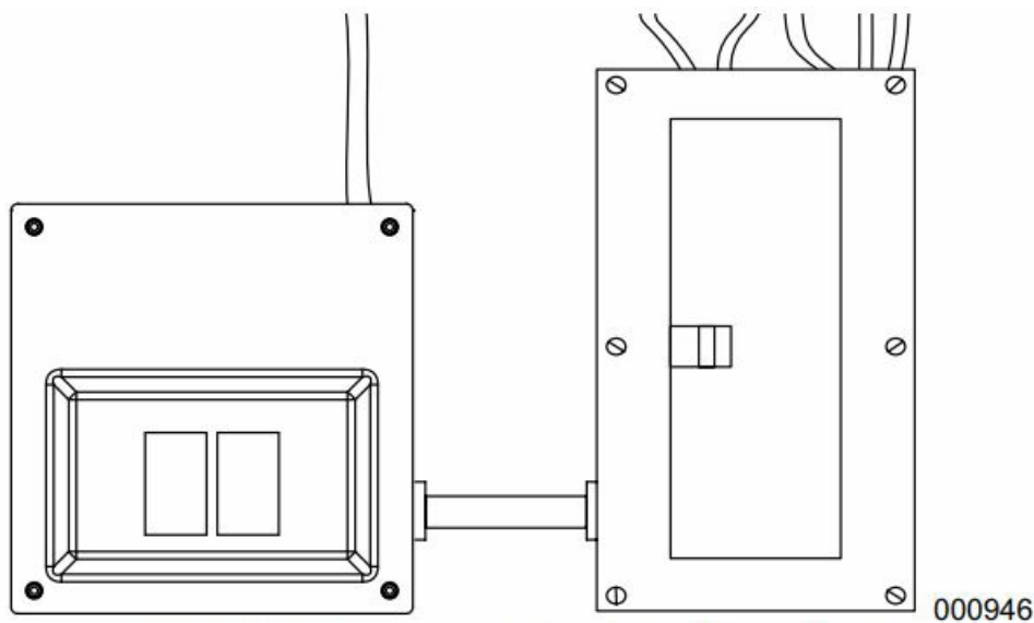
Figure 3-1. Transfer Switch Mounting
