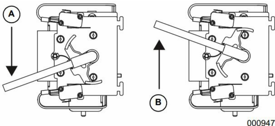
Figure 4-1. Transfer Mechanism Manual Operation
