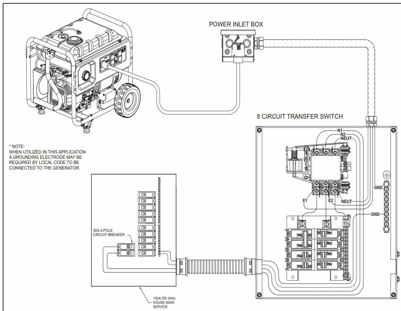
Interconnection Drawing No. 0K8844-C (Automatic Transfer Connections)
