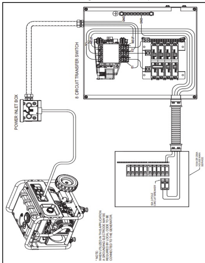
Interconnection Drawing No. 0K8845-A (Manual Transfer Connections)
