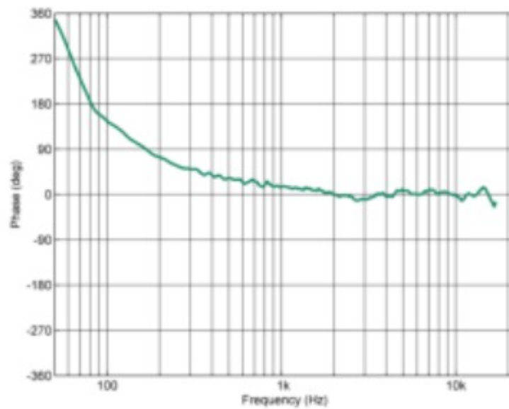
Figure 16. Phase response.
