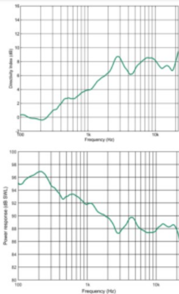
Figure 14. Directivity index (top) and power response (bottom).
