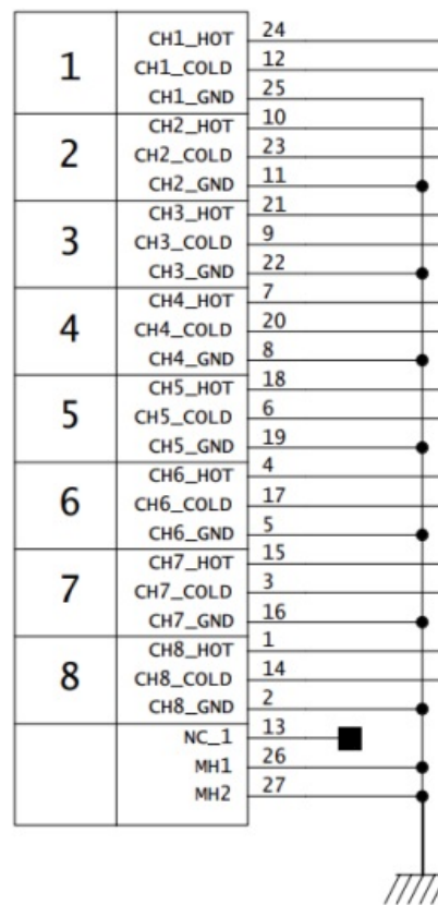
Figure 4. Digital audio output cable pin-out.
