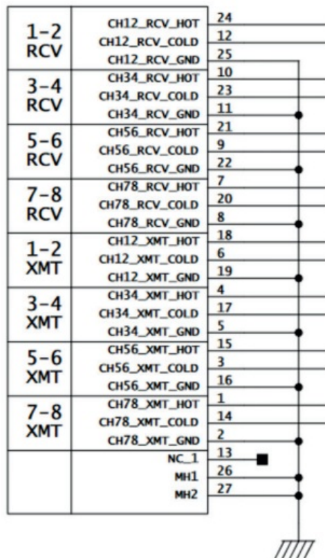
Figure 3. Digital audio input cable pin-out.
